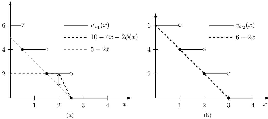
Figure 3: Illustration of the (Non-Linear) Cuts for the Second-Stage Cost Functions Derived in Example 2. The left figure displays the the second-stage cost function v_{\omega}(x) = 2[2.5 - x]^+ , and the non-linear cut v_{\omega_1}(x) \geq 10 - 4x - 2\phi(x) \forall x \in [0, 4] , where \phi(x) = \max\{0, 4 - 2x\} , x \in [0, 4] . Observe that this cut is tight at, e.g., \bar{x} = 2 , and strictly improves the best possible linear cut v_{\omega_1}(x) \geq 5 - 2x \forall x \in [0, 4] at \bar{x} . The right figure displays the second-stage cost function v_{\omega_2}(x) = 2[3 - x]^+ and the linear cut v_{\omega_2}(x) \geq 6 - 2x , which is tight at \bar{x} .
