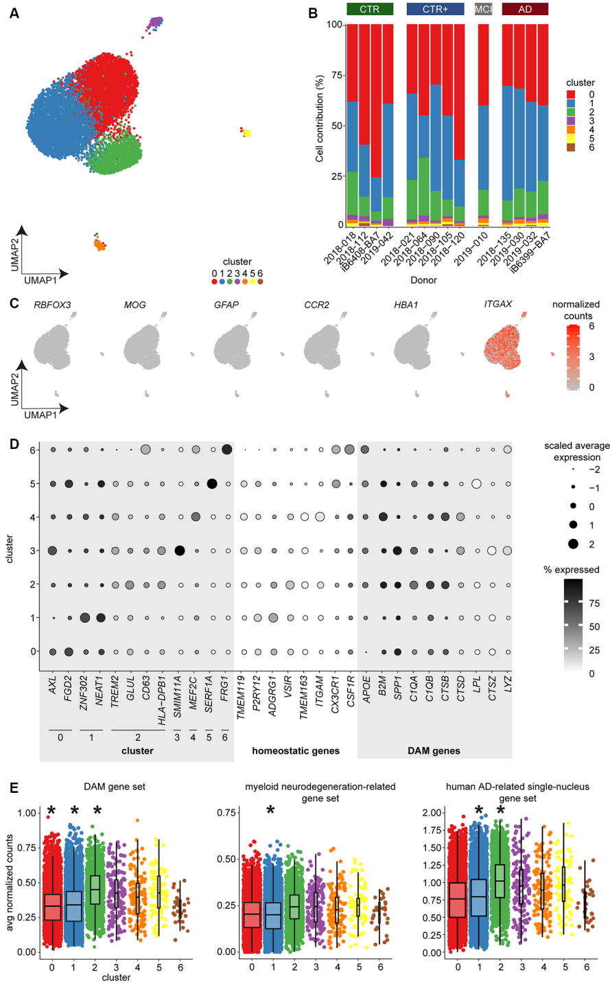
FIGURE 3 | Single-cell expression profiling of microglia identified seven subsets of microglia but no AD-associated cluster using bc-Smart-seq2. (A) UMAP visualization and unsupervised clustering of microglia derived from AD ( n = 4 ), MCI ( n = 1 ), CTR+ ( n = 5 ), and CTR ( n = 4 ) donors. Colors represent cluster identity. (B) Cluster contribution normalized to donor. (C) Expression of cell type-specific markers for neurons ( RBFOX3 ), oligodendrocytes ( MOG ), astrocytes ( GFAP ), circulating monocytes ( CCR2 ), erythrocytes ( HBA1 ), and microglia ( ITGAX ). (D) Dot plot visualizing scaled average expression and the percentage of cells expressing the indicated genes. (E) Average expression of the mouse DAM (Keren-Shaul et al., 2017), myeloid neurodegeneration-related (Friedman et al., 2018), and human AD-related single-nucleus (Mathys et al., 2019) gene sets per cell across clusters (multiple linear regression with Bonferroni correction, *indicate p -value < 0.001 ). Horizontal lines in the boxplots represent the mean; the lower and upper hinges represent the 25th and 75th percentiles. Abbreviations: AD, Alzheimer’s Disease; avg, average; CPM, counts per million; CTR, Control; CTR+, Control with A\beta plaques and/or hyperphosphorylated tau; DAM, disease-associated microglia; MCI, mild cognitive impairment; UMAP, uniform manifold approximation and projection.
