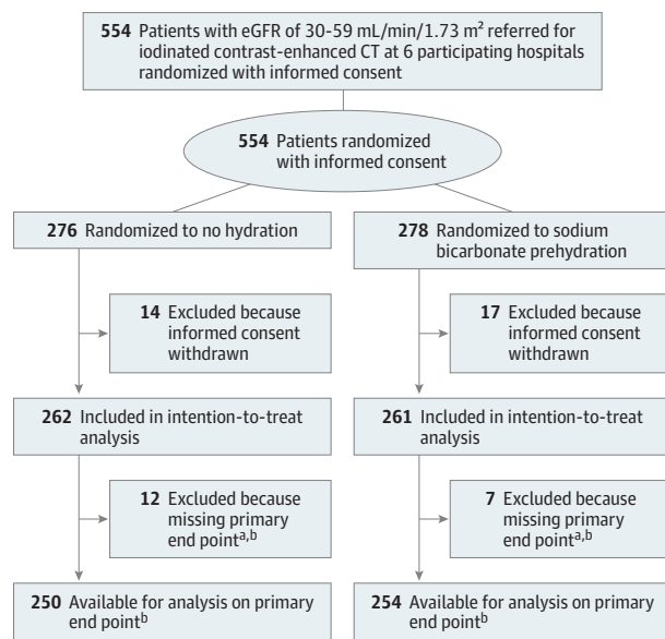
Figure 1. Trial Flowchart
