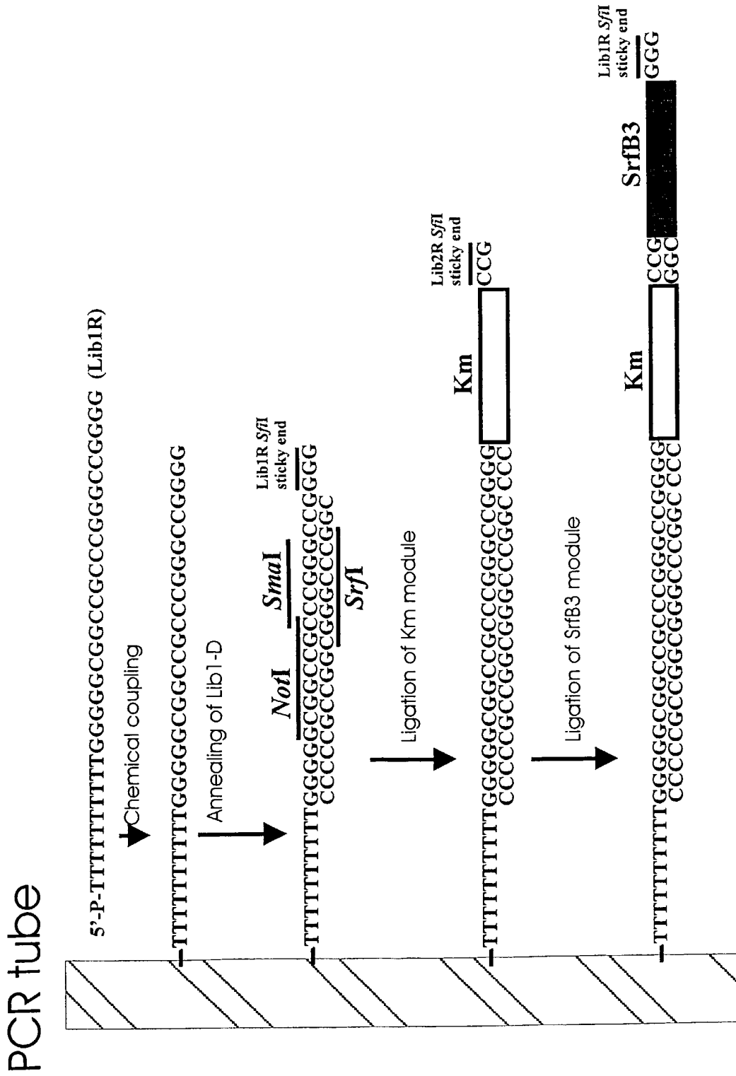
Fig. 19. Chemical coupling of oligo's to NucleoLink PCR tubes and the subsequent ligation of SfiI tagged modules.
