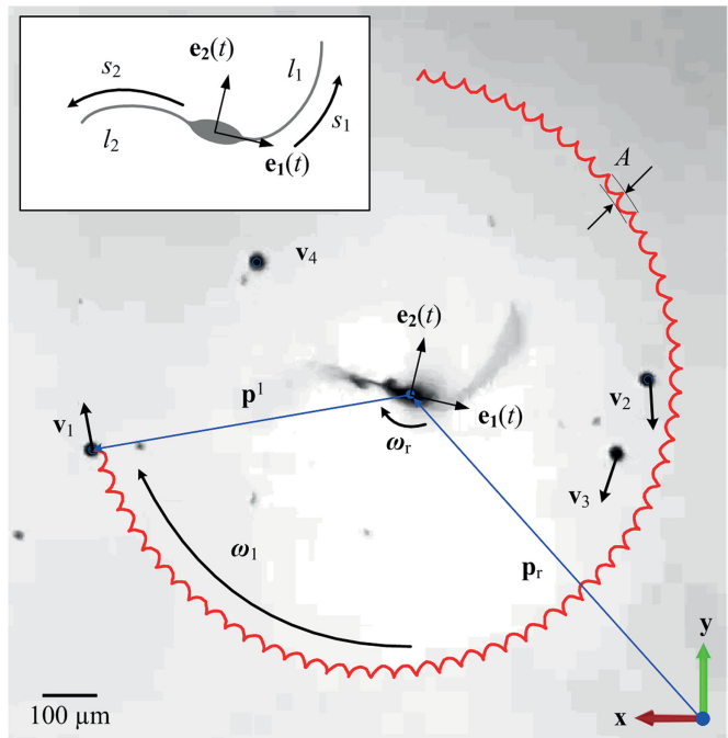
Fig. 1. Nonmagnetic microbeads orbit rotating two-tailed microrobot under the influence of its flow-field. The i th microbead moves at a linear velocity of v_i and p^i ( i = 1, \dots, 4 ) is its position vector from the two-tailed microrobot. e_1(t) and e_2(t) are orthonormal vectors of the material frame of the two-tailed microrobot. The sprocketlike trajectory (with amplitude A ) of the microbeads is generated by the asymmetric flow-field of the two tails of the microrobot. The tails have length of l_1 and l_2 and their shape is characterized by the deformation as a function of the arc length s_1 and s_2 . Rotation of the two-tailed microrobot at angular velocity \omega_r results in rotation of the i th microbeads at angular velocity of \omega_i .
