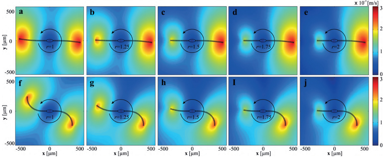
Fig. 2. Two-tailed microbot induces a flow-field during rotation under the influence of a rotating magnetic field. The flow-field is calculated using (9) and (11) for 2a = 50 \mu\text{m} , b = 20 \mu\text{m} , 2r_t = 5 \mu\text{m} , and \eta = 0.95 \text{ Pa}\cdot\text{s} . (a)–(e) Flow-fields of two-tailed rigid microbots are calculated for tail length ratios of 1, 1.25, 1.5, 1.75, and 2. (f)–(j) Flow-fields of two-tailed flexible microbots (modulus of elasticity of 0.54 GPa) are calculated for tail length ratios of 1, 1.25, 1.5, 1.75, and 2. The flow-field created by the rigid microbots is slightly higher than the flow-field of the soft microbot regardless to the tail length ratio.
