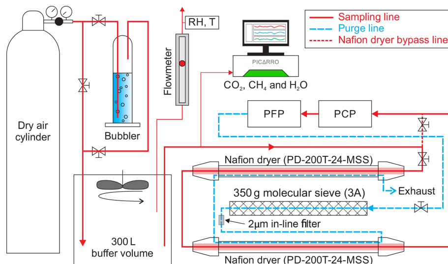
Figure 5. Schematic of the setup used at INSTAAR to determine the effect of the NAD on the mole fraction determination of CO, CH 4 , N 2 O and SF 6 along with CO 2 and its singly substituted isotopologues. A NOAA-ESRL PCP–PFP system could be flushed with either dry or humidified cylinder air including or bypassing the NAD. Flow from the cylinder was adjusted such that there was always an overflow of air from the buffer volume, where relative humidity of the sample was constantly monitored. A Picarro analyzer was used to monitor the stability of CO 2 , CH 4 and H 2 O mole fractions in the gas exiting the buffer volume, during all the tested experimental conditions, a summary of which is shown in Fig. 6.
