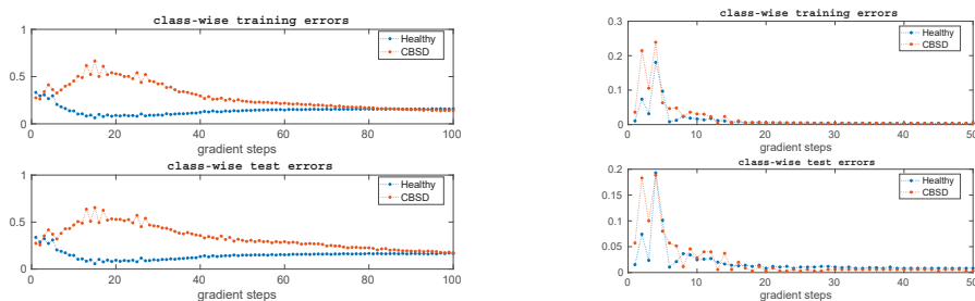
Figure 6.5: Class-wise training error in original space (left) and PCA (right)
