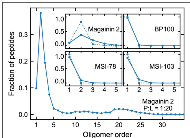
FIGURE 4 | Oligomerization preference of each peptide, analyzed over the last 20 \mu s of simulation and expressed as the fraction of the total peptide per oligomer order. Main plot: distribution for Magainin-2 at high (P:L = 1:20) concentrations. Insets: distributions for all the peptides, at P:L ratios of 1:200 (dotted line) and 1:20 (full line), with plots focused on low oligomerization numbers.
