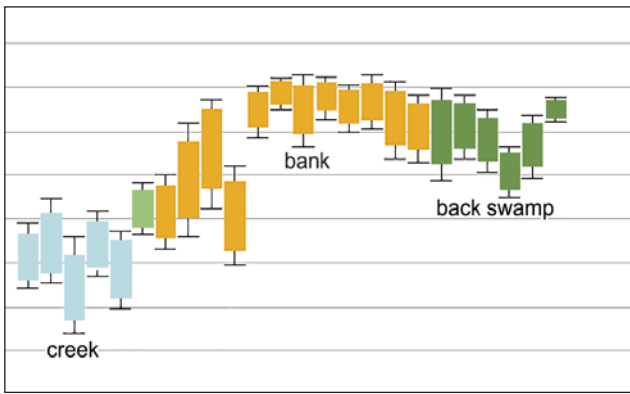
Fig. 6.3 A vertical flip of a series of boxplots displaying the range in moisture values for taxa commonly present in modern syntaxa as identified from the drift litter samples, resulting in a visual match closely approaching the known geomorphology of the banks (see chapter 2). The colour scheme follows the field guide of Dutch plant communities (Schaminée et al. , 2010). Blue: open water and marsh. Light green: grassland and heathland. Orange: coastal and inland pioneer communities. Dark green: thicket and woodland. Figure produced via SynBioSys (Hennekens et al. , 2010) based on indicator values presented in Ellenberg et al. , (1991).
