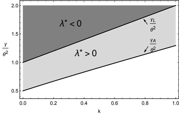
Figure 1: The sign of \lambda^* in the feasible parameter area characterized by \gamma > \gamma_A (given any \theta > 0 ).
