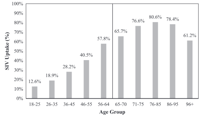
Fig. 2. SIV uptake (%) across all seasons 2011–2016 stratified by age groups.
