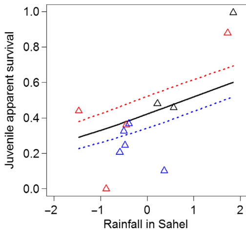
Figure 3. Relationship between apparent juvenile survival and the amount of rainfall during the rainy season in the western Sahel (standardised values) for 12 cohorts of Montagu's harriers tagged between 1988 and 1999 in Rochefort. Estimates were taken from models c1 (Table 1). This model also includes an additive effect of average annual breeding success. Black, red and blue lines indicate predicted values for the average, the first and third quartiles of average annual breeding success, respectively. Triangles present annual juvenile survival estimates from a time-dependent model without any covariate (same as in Fig. 1; model c14). Their colour refers to the categorisation described above.
