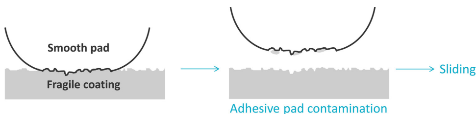
Fig. 1. Schematic showing the contamination mechanism of smooth adhesive pads on slippery, fragile surfaces.
