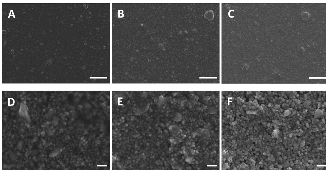
Fig. 4. SEM images of 30 wt% TiO 2 , 20 wt% CaCO 3 paint surfaces with varying PVC: (A, D) PVC 50, (B, E) PVC 60 and (C, F) PVC 70. Paints shown in (B, E) and (C, F) are formulated above their CPVC. Scale bars: (A–C) 100 μm and (D–F) 1 μm.
