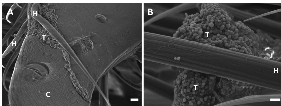
Fig. 2. SEM images from Atta cephalotes tarsi after walking on a wall painted with Fluon coating (Blades Biological Ltd, Edenbridge, UK). Fluon is a slippery coating used to retain insects in their nest containers. Some areas of (A) claws and (B) tarsus' hairs are covered in PTFE particles. Labels: H: hairs, T: PTFE, C: claw. Scale bars: 1 \mu\text{m} .
