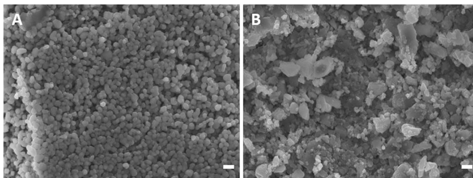
Fig. 3. SEM images of the (A) titanium dioxide (Tiona 595, spherical shape, mean diameter: 300 nm) and (B) calcium carbonate (Omyacoat 850-OG, platelet shape, mean diameter: 1 \mu\text{m} ) grades used in this study. Scale bars: 1 \mu\text{m} .
