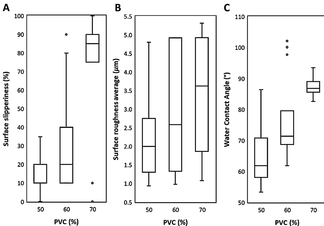
Fig. 5. Boxplots showing (A) surface slipperiness (percentage of unsuccessful ants in climbing tests), (B) surface roughness average ( R_a ) and (C) water contact angle measured for the full set of paints formulated at different PVC values. In (B), three outliers ( R_a > 10 \mu\text{m} ) were not shown for more clarity. Centre lines and boxes represent the median within the 25th and 75th percentiles, whiskers show the 10th and 90th percentiles and circles indicate outliers.
