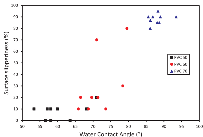
Fig. 7. Contact angle of water on paint surface vs. slipperiness (portion of unsuccessful ants) and PVC. One can see that both slipperiness and water contact angle increased with PVC. Data points corresponding to \text{TiO}_2 - and \text{CaCO}_3 -only paints and error bars were not included for more clarity.
