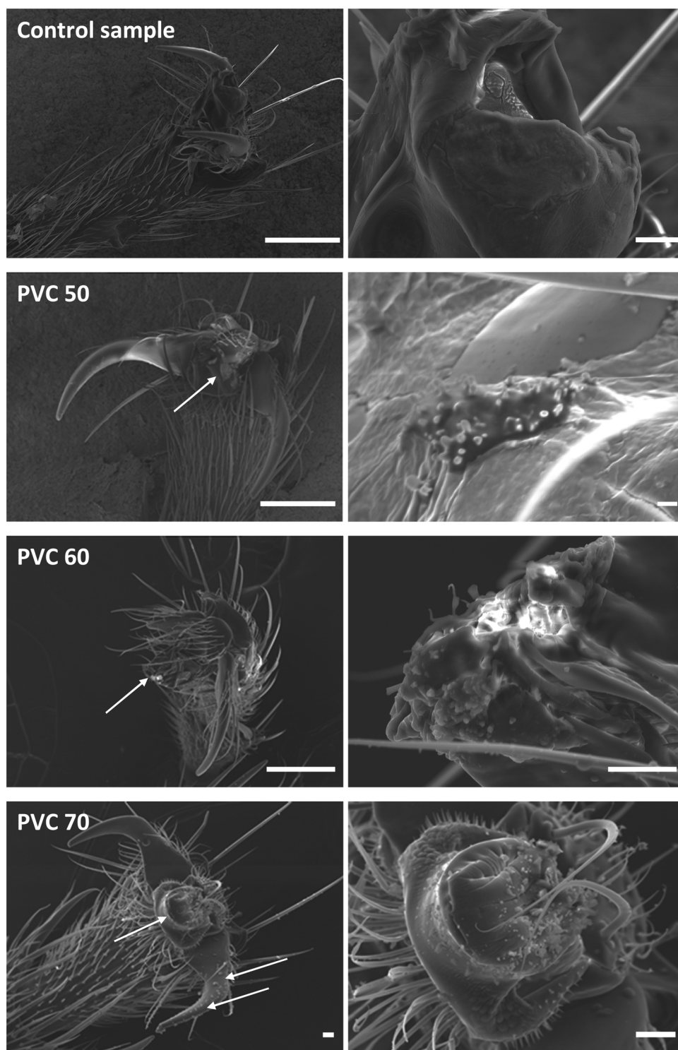
Fig. 8. SEM images of A. cephalotes ant tarsi contamination after climbing 30 wt% \text{TiO}_2 , 20 wt% \text{CaCO}_3 paint surfaces formulated at PVC 50, 60 and 70. Control sample: ants which did not climb on paint, no contaminants could be observed. Scale bars: 100 \mu\text{m} (left) and 10 \mu\text{m} (right). PVC 50: only a few contaminating particles could be observed on the arolium; scale bars: 100 \mu\text{m} (left) and 1 \mu\text{m} (right). PVC 60: the arolium tip was fouled by paint particles. Scale bars: 100 \mu\text{m} (left) and 10 \mu\text{m} (right). PVC 70: the arolium and claws were heavily contaminated by particles, mostly \text{CaCO}_3 . Arrows show contaminating particles. Scale bars: 10 \mu\text{m} (left) and 10 \mu\text{m} (right).
