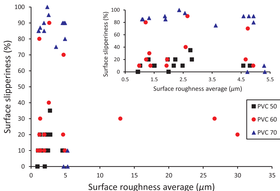
Fig. 6. Surface slipperiness (percentage of unsuccessful ants) of model paints formulated at different PVCs vs. surface roughness average R_a for PVCs 50, 60 and 70; inset: detail of 0.5–5.5 \mu\text{m} roughness. It can be seen that an effect of R_a on slipperiness cannot directly be concluded from this graph. Error bars are not included for more clarity.
