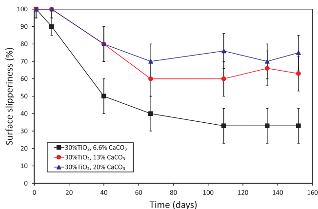
Fig. 11. Long-term slipperiness test: slipperiness (portion of unsuccessful ants) measured as a function of time during 5 months by leaving the painted panels (30% TiO 2 , variable concentration of CaCO 3 ) in the A. cephalotes colony's rearing. A slipperiness plateau was reached within ca. 2 months for the three paints, which suggests that thereafter, insect attachment forces were reduced through surface roughness.
