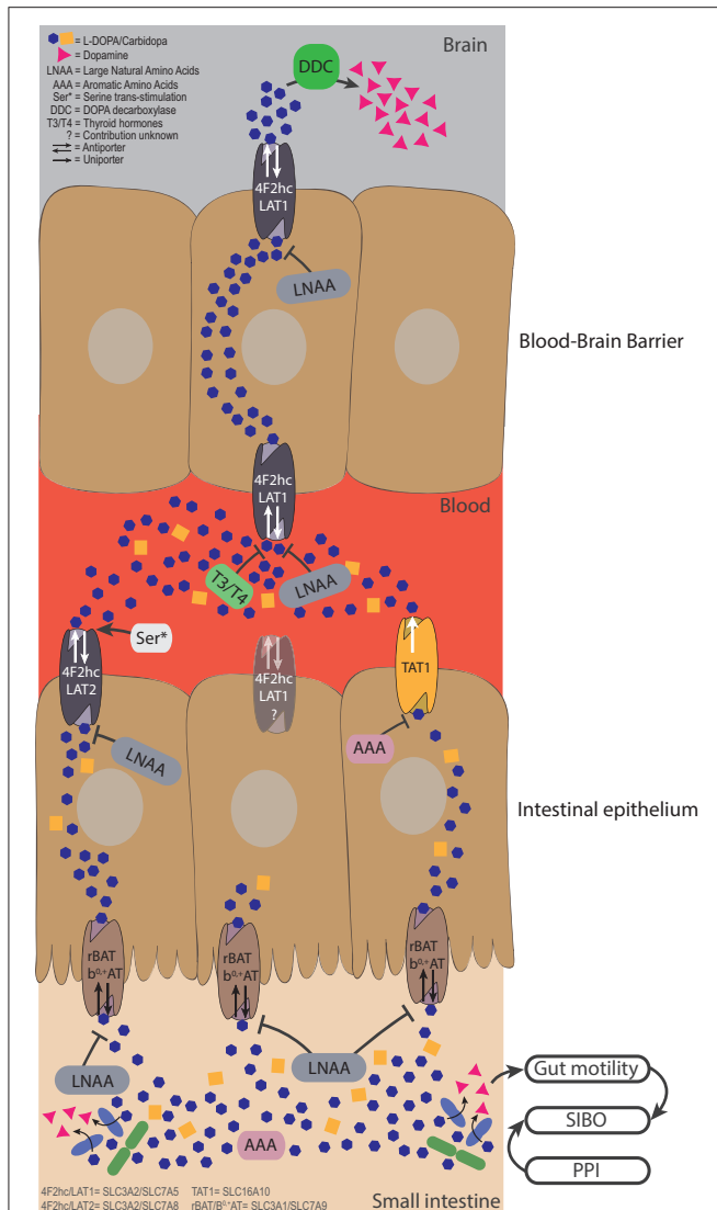
FIGURE 2 | Bacterial degradation and dietary components restrict levodopa transport. Levodopa is taken up in the small intestine by the apical transporter rBAT/b 0,+ AT, and is sequentially is transported over the basolateral membrane by 4F2hc/LAT2 and TAT1. The uptake from the lumen can be compromised by LNAA apically and by LNAA and AAAs basolaterally. Bacterial degradation can interfere with levodopa before it is transported and elevate levels of dopamine in the lumen. Higher levels of luminal dopamine could affect the gut motility, which, in turn, could result in a state of small intestinal bacterial overgrowth, creating a vicious circle. The fraction of levodopa that ends up in the blood has to be transported over the BBB via 4F2hc/LAT1, which can be compromised by high levels of thyroid hormones (T3/T4), or LNAA. Serine left over from a late proteic meal, can trans-stimulate 4F2hc/LAT2 inducing higher efflux of levodopa in the circulation. Finally, the remaining levodopa will be converted to dopamine in the brain by DDC, to compensate the loss of striatal dopamine levels in PD patients.
