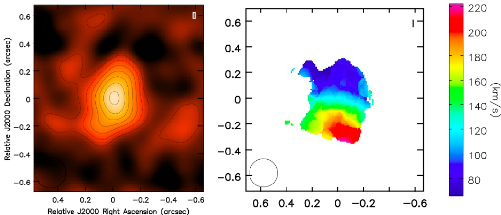
Figure 2. (Left:) A simulated image of the velocity integrated [CII] 158 \mu\text{m} emission from a z = 15 galaxy with a star formation rate of 5 M_{\odot} \text{yr}^{-1} , and a metallicity of 0.2 Z_{\odot} , assuming for a 40 hr observation with the ngVLA. The contour levels are -6, -3, 3, 6, 9, 12, 15, 18, 21 \mu\text{Jy beam}^{-1} . The rms noise on the image is about 1.8 \mu\text{Jy beam}^{-1} , and the synthesized beam FWHM is 0''.22 . (Right:) The intensity weighted mean [CII] velocity (moment 1).
