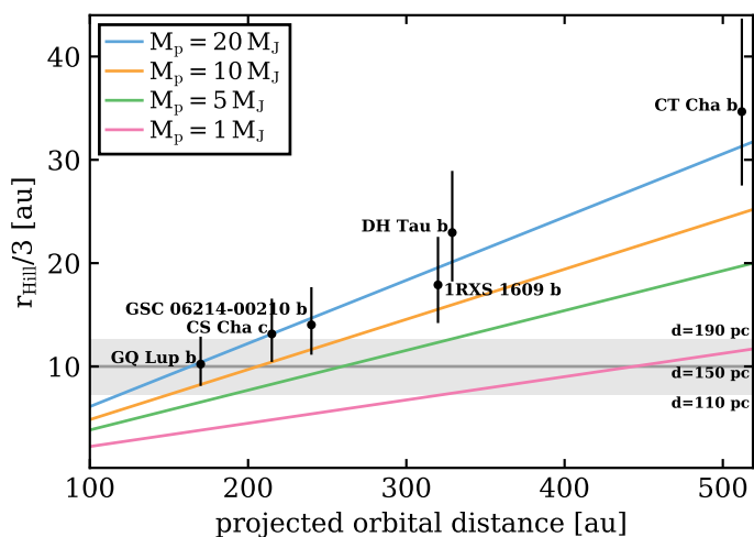
Fig. 10. One-third of the Hill radius ( r_{\text{Hill}}/3 ) vs. orbital distance for a selection of detected PMCs (black symbols) and as reference for companions orbiting a solar-mass star (coloured lines, 4 different PMC masses). We note that for example the curve for M_p = 20 M_J is identical to the curve for a M_p = 10 M_J companion but around a 0.5 M_\odot star. The thick grey horizontal line and the grey box indicate the detection limit for the gas disk of r = 10 \pm 2.7 au for distances of 110 – 190 pc. The error bars indicate a factor of two uncertainty in the mass of the companion; the real error might be significantly larger.
