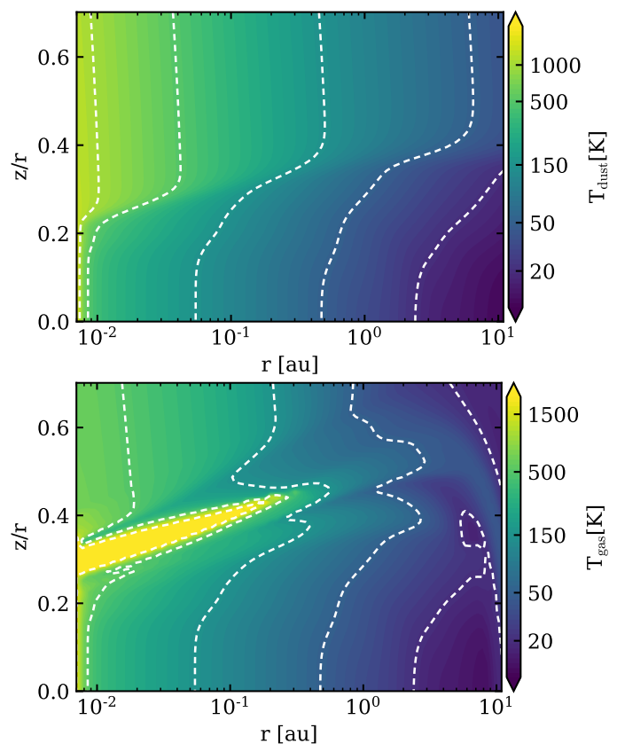
Fig. B.1. Dust (top panel) and gas (bottom panel) temperature structure for the reference model (see Sect. 2.1). The white dashed contour lines correspond to the temperature values given in the colour bar. The logarithmic colour scale is the same in both plots.
