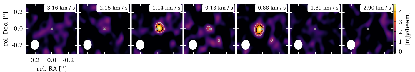
Fig. 9. ^{12}\text{CO } J=3-2 (ALMA B7) synthetic channel intensity maps for a CS Cha companion model. The grey cross indicates the location of the PMC. The white ellipse in each panel shows the beam with a size of 0.11'' \times 0.09'' . In the top right corner of each panel the velocity relative to the systemic velocity is indicated. The grey and black contours show 3 and 5 times the theoretical rms level of 0.65 mJy/beam (see Table C.1). The measured rms levels in the shown channels are approximately in the range 0.49 – 0.76 mJy/beam. The measured peak flux is about 4.8 mJy/beam.
