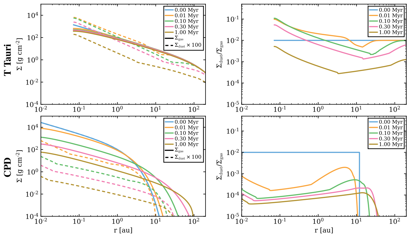
Fig. F.1. Results from the two-pop-py dust evolution model. The top row represents a T Tauri disk model; the bottom row shows the reference CPD model. The left column shows the time evolution of the gas (solid lines) and dust (dashed lines) surface densities as a function of radius; the right column shows the evolution of the dust-to-gas mass ratio.
