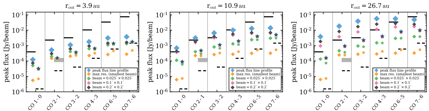
Fig. 11. Impact of the beam size on the observed fluxes. Each individual panel shows the same kind of plot as shown in Fig. 5. In each panel one model with a certain disk extension is shown. For each of these models, the peak fluxes using different beam sizes are reported (coloured symbols in each panel). As a reference also the given line peak flux (blue diamonds) as derived from the line profile is shown (i.e. is not per beam). For the continuum, the big blue stars show the total integrated flux.
