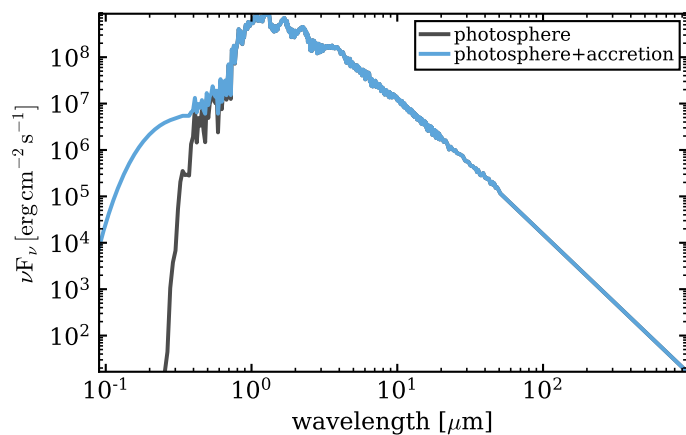
Fig. 1. Spectrum for our reference PMC with M_p = 20 M_J . The solid black line indicates the photospheric (intrinsic) spectrum and the blue line shows the spectrum with the added accretion luminosity.
