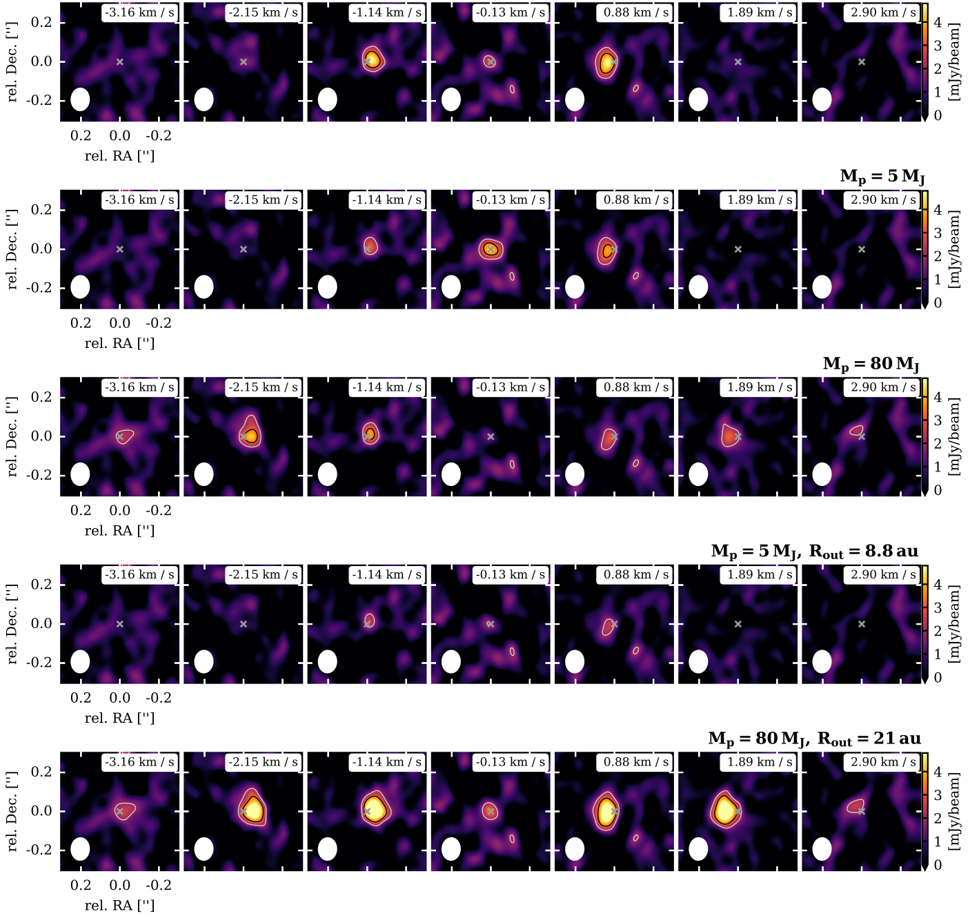
Fig. G.1. ^{12}\text{CO } J = 3 - 2 (ALMA Band 7) synthetic channel intensity maps for CS Cha companion models. The grey cross indicates the central target location. The white ellipse in each panel shows the beam with a size of 0.11'' \times 0.09'' . In the top right corner of each panel the velocity relative to the systemic velocity is indicated. The grey and black contours show 3 and 5 times the theoretical rms level of 0.65 \text{ mJy/beam} (see Table C.1). In the top row we show the same model as in Fig. 9 (Sect. 3.5) for easier comparison. The second and third row show models where only the PMC mass was changed. For the models in the last two rows the disk outer radius was adapted to r_{\text{Hill}}/3 according to the PMC mass. The spatial and colour scale are the same for all five plots.
