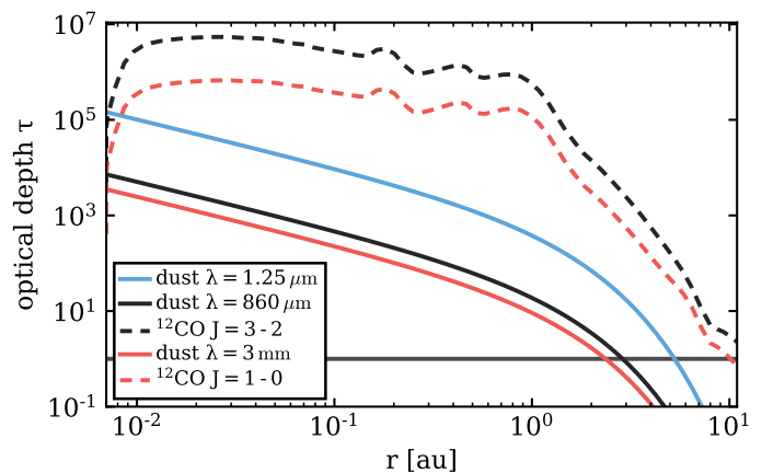
Fig. 4. Vertical optical depth \tau for the dust and for ^{12}\text{CO} lines as a function of radius in the reference model (see also Fig. 3). The horizontal dark grey line indicates \tau = 1 .
