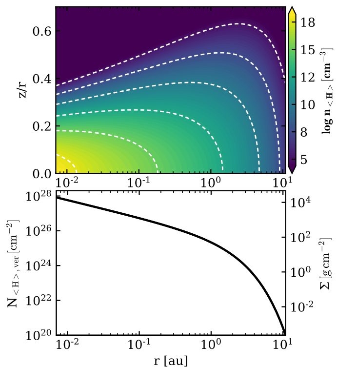
Fig. 2. Gas disk structure of the reference CPD model. The top panel shows the total hydrogen number density n_{\text{H}} . The height of the disk z is scaled by the radius r . The white dashed contours correspond to the density levels shown in the colour bar. The bottom panel shows the total vertical hydrogen column number density N_{\text{H},\text{ver}} as a function of radius; the scale for the surface density \Sigma in \text{g cm}^{-2} is given on the right-hand side.
