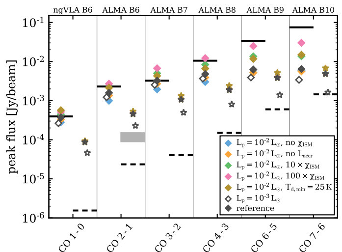
Fig. 7. Same as Fig. 5 but for models with varying radiation properties of the PMC and the environment (background field). The underlying disk structure is always that from the reference model.
