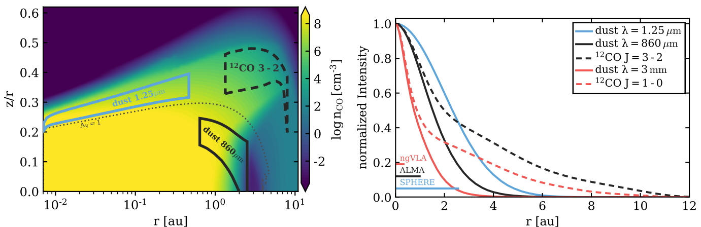
Fig. 3. Left panel: Location of the main emitting region for the near-infrared and (sub)mm dust emission and the ^{12}\text{CO } J=3-2 line in the reference model. The vertical lines of the boxes denote the radii where the cumulative flux in radial directions reaches 15% and 85%, respectively. The horizontal lines denote the heights where the cumulative flux integrated vertically reaches 15% and 85% at each radial position. The coloured contours show the CO number density and the dotted grey line shows where the visual extinction A_V reaches unity. Right panel: Normalized radial intensity profiles (azimuthally averaged) for the dust continuum and line images. Shown are profiles derived from images convolved with representative beam sizes for SPHERE (blue, FWHM = 0.031"), ALMA (black, FWHM = 0.012"), and ngVLA (red, FWHM = 0.004").
