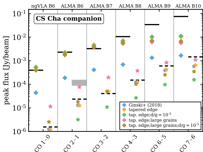
Fig. 8. Same as Fig. 5 but for the CS Cha companion model. Shown are the original Ginski et al. (2018) model and several tapered-edge models with different dust-to-gas mass ratios ( d/g ) and dust compositions/populations (large grains).
