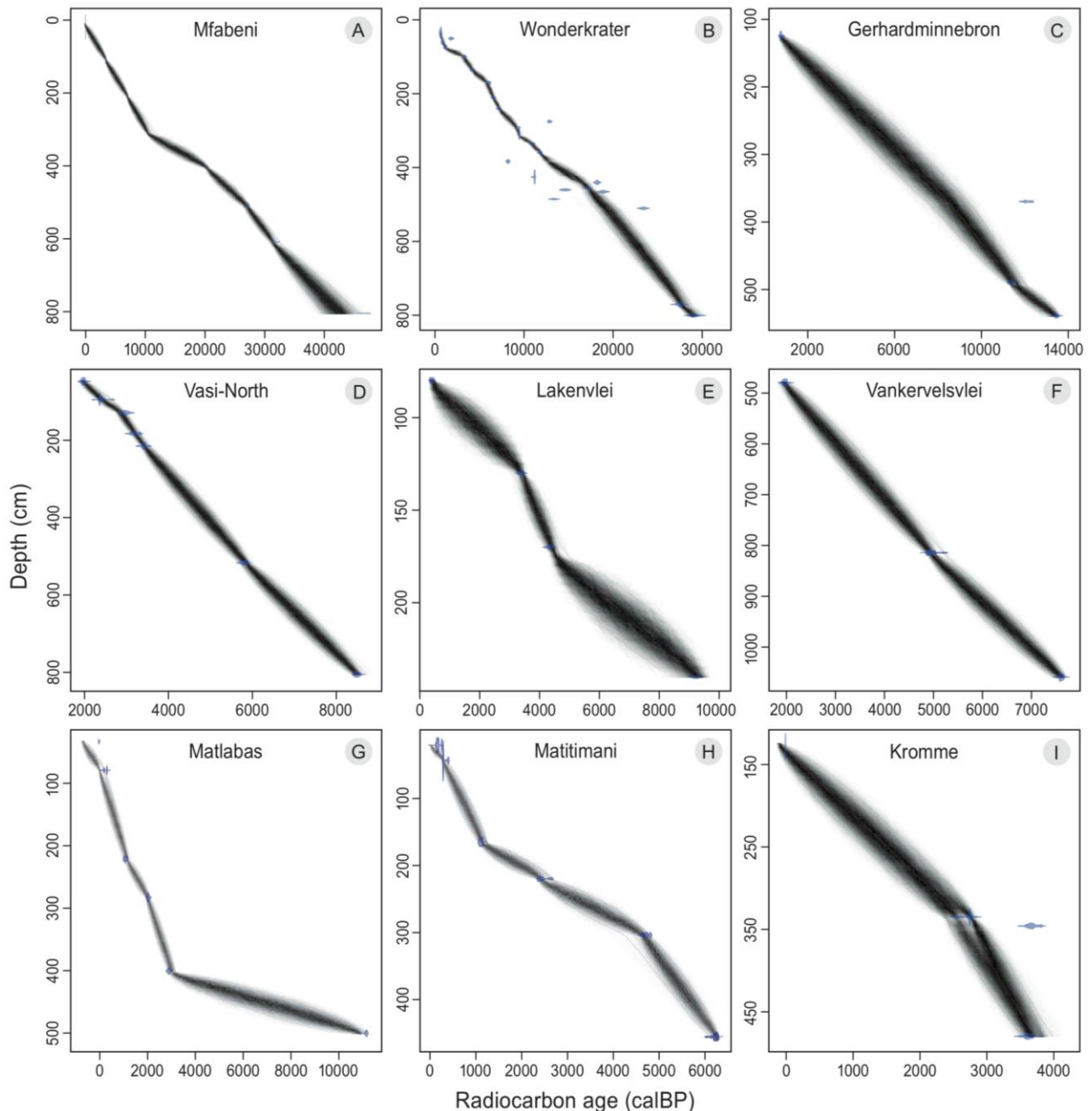
Figure 5. Age-depth models for nine peatlands in South Africa. The blue ranges represent the calibrated sample age ranges while the black shadows represent the calibrated range of each point interpolated between the sampled ages (calBP cm -1 ). calBP = radiocarbon calibrated calendar age. A: adapted from Baker et al. (2014); B: adapted from Scott et al. (2003); C–I: data collected during this study.
