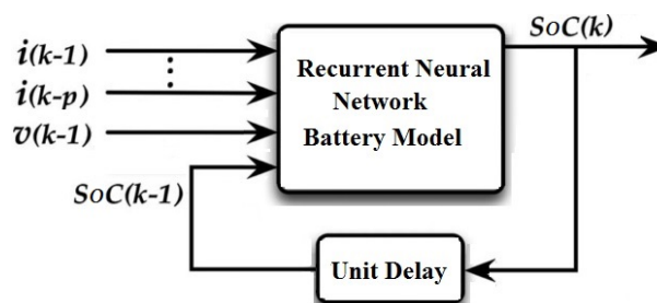
Figure 1: A sample structure of the recurrent neural network for state of charge estimation in the Li-ion batteries
