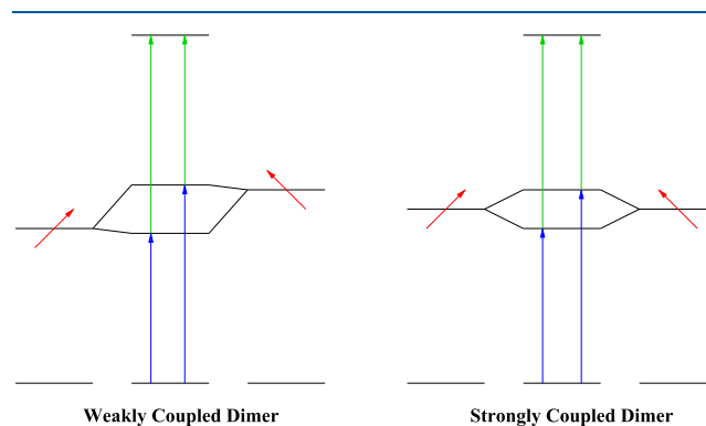
Figure 9. Energy diagrams for the employed dimer models. Left: Weakly coupled dimer. Right: Strongly coupled dimer. The black lines indicate the energy levels of the individual chromophores coupled to form the composite dimer energy levels in the middle. The red arrows indicate the directions of the transition dipole moments of the monomers, and the vertical blue and green arrows indicate the transitions in the dimer systems.
