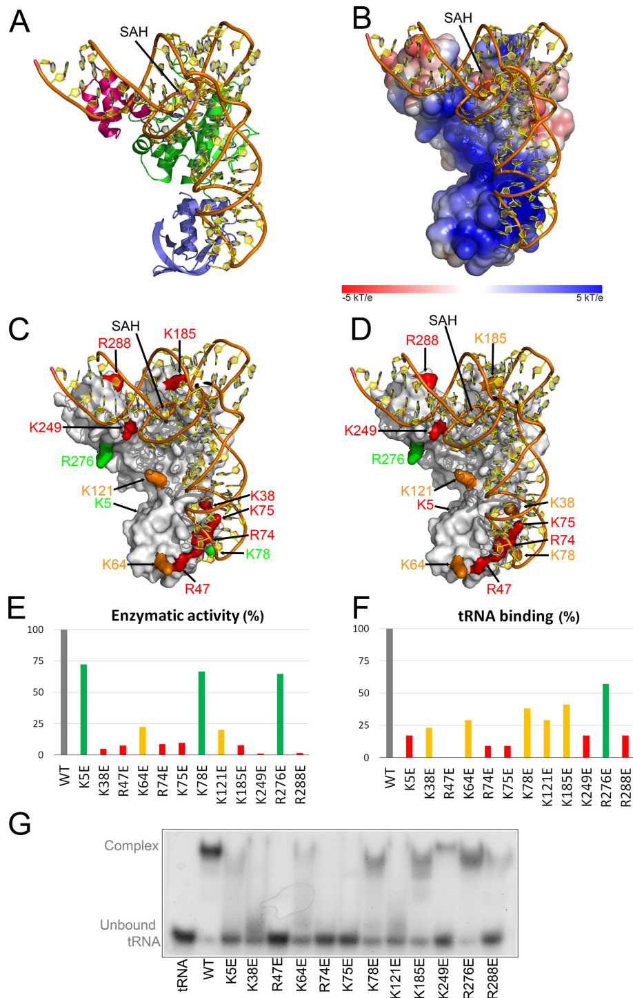
Figure 3. Docking model of tRNA Met of S. acidocaldarius onto Sa Trm10_SAH (model 2). For S. acidocaldarius tRNA Met a homology model based on the structure of E. coli tRNA Met was used. (A) Docking model 2 with both tRNA Met and Sa Trm10_SAH shown in cartoon representation. The N-terminal, SPOUT and C-terminal domains of Sa Trm10 are coloured blue, green and pink, respectively. (B) Docking model 2 in the same orientation as in (A) with Sa Trm10_SAH shown with the electrostatic potential mapped on its solvent accessible surface. (C and D) Results of the mutagenesis data, as evaluated with a tRNA methylation assay (C) and EMSA measurements (D), mapped on the surface of docking model 2 (an SDS-PAGE of these protein variants is shown in Supplementary Figure S6). The residues that have been substituted to validate the docking model are coloured according to the results of the tRNA methylation assay (C) or EMSA (D) using the following colour code: green: 50–100% activity/binding compared to WT; orange: 50–20% activity/binding compared to WT; red: 20–0% activity/binding compared to WT. (E, F and G) Results of the tRNA methylation assay using [methyl- 14 C]SAM (E), and of the single concentration EMSA (F and G) of protein variants that were generated in this study to validate the docking model. Panel F displays the fraction of bound tRNA normalized against the wild type protein, as determined from the EMSA shown in panel G. Hereto, the density of the band corresponding to unbound tRNA was measured and compared to the band in absence of protein (labelled 'tRNA'). The value of the wild type protein was set as 100%. Residues Lys5 and Lys78 were chosen away from the proposed binding surface to serve as negative controls.
