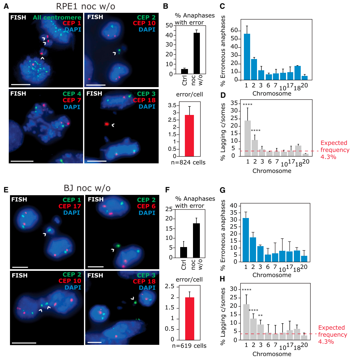
Figure 2. Chromosomes 1 and 2 Are Highly Prone to Lagging After Nocodazole Washout
