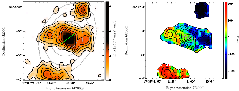
Figure 5.4 – (a): Intensity map of the H 2 1-0 S(1) line in the inner 2 kpc of PKS B1718-649. The position angle of the radio source is shown in dashed green (PA= 135°). Intensity contours at 1.5, 3, 5, 7, 9, 12, and 15-σ are shown in black, starting from 1.5σ = 2.5 × 10 -17 erg s -1 cm -2 . The isophotes in grey show the distribution of the stellar component. (b): Velocity field of the H 2 1-0 S(1) line with the contours of the intensity map overlaid. The position angle of the radio source is shown in black. Velocities are given relative to the systemic value, v sys = 4274 km s -1 . The regions marked by crosses are those where we extracted the profiles of Fig. 5.5, (see the text for more details).
