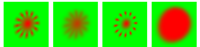
Figure 5: Comparing the blending weights of \mathcal{A}_1 \dots \mathcal{A}_4 (left to right) for a once-subdivided polar configuration (EV with a high valency, n = 12 , surrounded by triangles). \mathcal{A}_3 has to be subdivided once more before the weights can be initialised.
