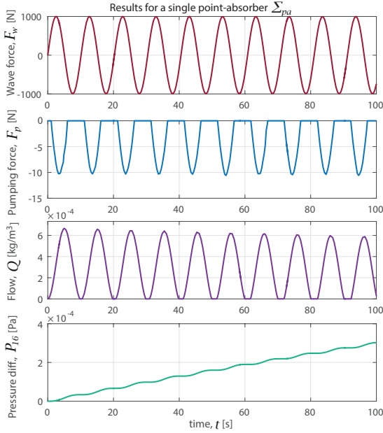
Fig. 5. Incoming wave force F_w , pumping force F_p , volumetric flow Q , and pressure difference P_{16} for \Sigma_{pa} .
