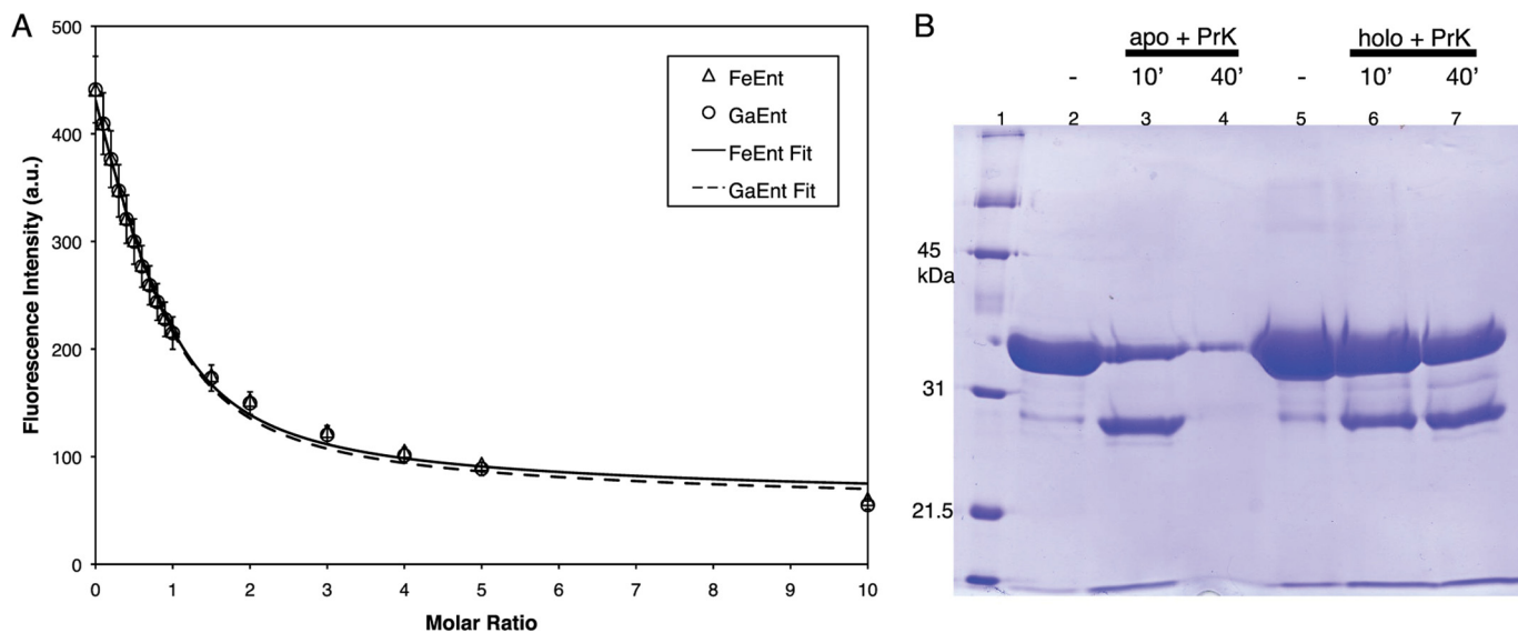
FIGURE 6. FeEnt and GaEnt binding properties of FepB. A , fluorescence spectroscopy titration of FepB with FeEnt and GaEnt. The fluorescence intensity in arbitrary units ( a.u. ) at 330 nm decreases upon the addition of ligand. Each addition of GaEnt (○) and FeEnt (△) is shown. The curve fits for the determination of K_D are also depicted. All experiments were performed in triplicate. B , proteinase K protection assays of FepB with and without GaEnt were run on a 12% SDS-PAGE. Identical results were also obtained with the FeEnt-FepB complex (data not shown). Lane 1 , low range molecular weight markers; Lanes 2 and 5 , controls for FepB and GaEnt-FepB without proteinase K ( PrK ). Lanes 3 and 4 , FepB after 10 and 40 min of proteinase K digestion, respectively. Similarly, lanes 6 and 7 are GaEnt-FepB after 10 and 40 min of digestion, respectively.
