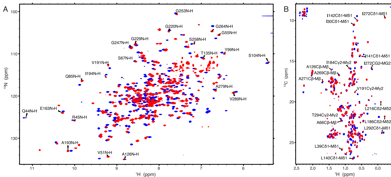
FIGURE 2. NMR spectra of apo (red)- and holo-FepB (blue). In A, overlaid U- ^{15}\text{N} ^2\text{H}/^1\text{H} -labeled apo- and holo-FepB ( \sim 1 mM) spectra from a ^1\text{H} - ^{15}\text{N} TROSY-HSQC experiment. In B, overlaid U- ^{13}\text{C} , ^{15}\text{N} ^2\text{H}/^1\text{H} -labeled apo- and holo-FepB ( \sim 1 mM) spectra from a \text{CHD}_2 -detected CT- ^1\text{H} - ^{13}\text{C} HSQC experiment. All experiments were acquired in 50 mM \text{Na}_3\text{PO}_4 (pH 6.4) at 298 K on a 700 MHz ( ^1\text{H} - ^{15}\text{N} TROSY-HSQC) or 600 MHz (CT- ^1\text{H} - ^{13}\text{C} HSQC) NMR spectrometer. Several residues that could be clearly labeled and with adjacent apo- and holo-peaks are indicated.
