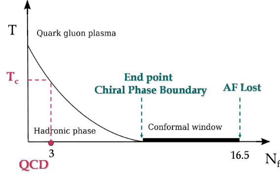
Figure 1: A qualitative view of the phase diagram of a QCD-like gauge theory with varying flavor content, in the T, N_f plane.
