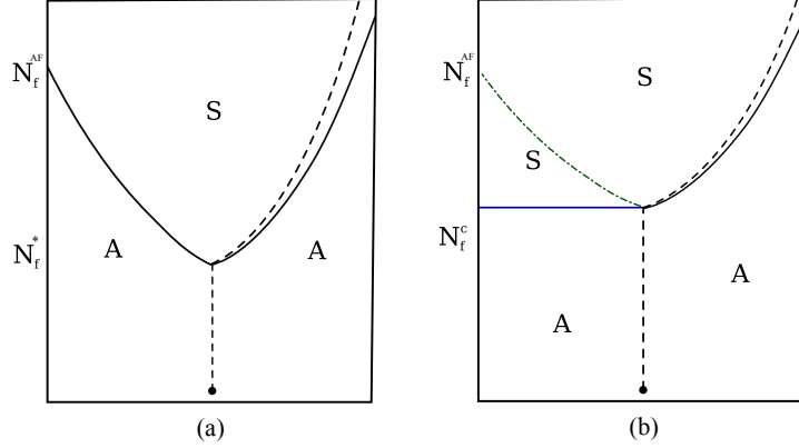
Figure 3: (a) The Banks-Zaks scenario for conformal symmetry restoration [6] by varying the gauge coupling g and flavors N_f . S and A refer to chirally symmetric and asymmetric, respectively. Dashed lines are chiral transitions and solid lines are confinement transitions. They coincide on the left branch, location of the IRFP. (b) The modified scenario by [8]. The horizontal (blue) line is the conformal phase transition (CPT) that opens up the conformal window. The dot-dashed (green) line is the location of the IRFPs.
