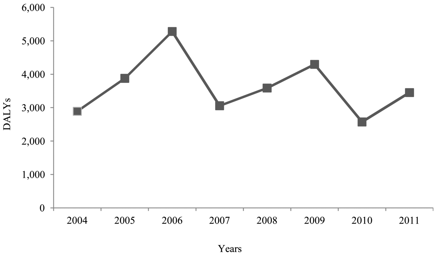
Fig 3. Trend analysis of TBE burden expressed in total DALYs in years 2004 to 2011 from the population perspective.
