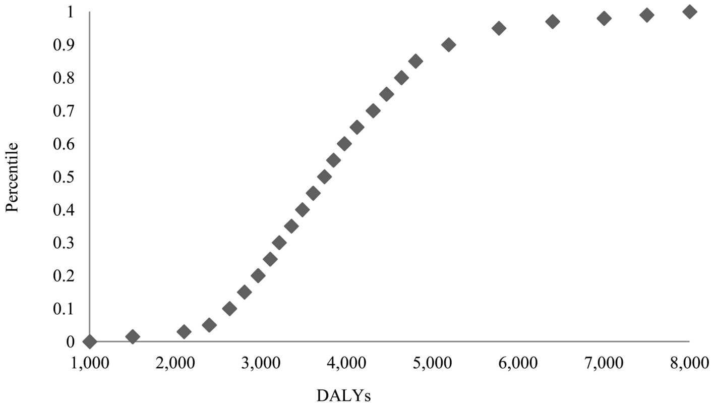
Fig 5. Cumulative ascending curve of the probabilistic sensitivity analysis of TBE burden expressed in total DALYs from the population perspective, reflecting the likelihood (y-axis) of being below a specified total DALYs impact (x-axis).
