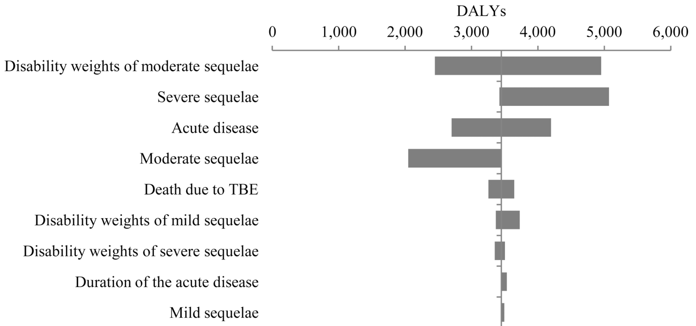
Fig 4. Tornado diagram of the one-way sensitivity analyses of TBE burden expressed in total DALYs from the population perspective.
