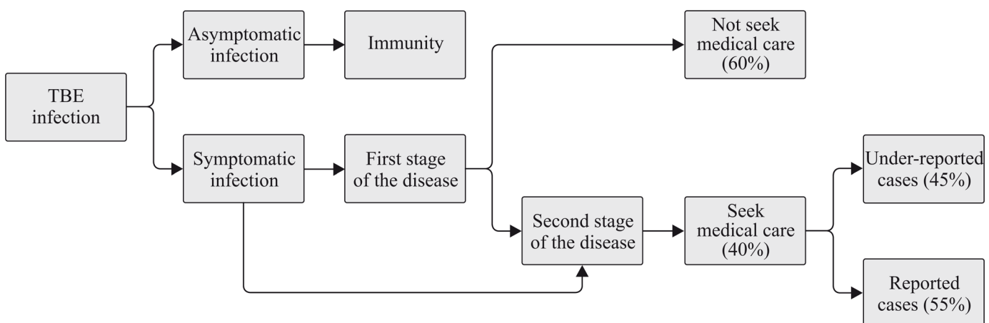
Fig 1. Schematic presentation of disease progression, used to estimate the factors \beta_r , \beta_a and consequently \gamma ; with \gamma (4.5) to correct under-estimation of the reported number of cases with the acute disease of the second stage ( n_{ra} ) resulting from the product of a factor \beta_a ( 100/40 = 2.5 ) to correct for under-ascertainment and a factor \beta_r ( 100/55 = 1.8 ) to correct for under-reporting.
