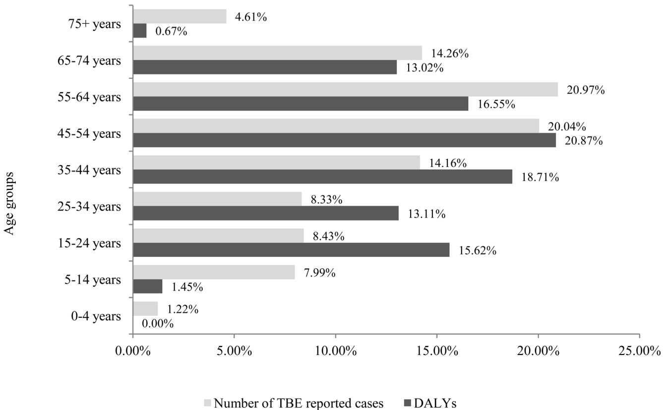
Fig 2. Comparison of relative TBE burden expressed in total DALYs from the population perspective with the relative TBE burden expressed by the number of reported cases by age groups. DALYs and reported cases are averages over 2004–2011.
