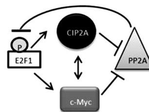
Figure 1. CIP2A/c-Myc/E2F1 pathway.
