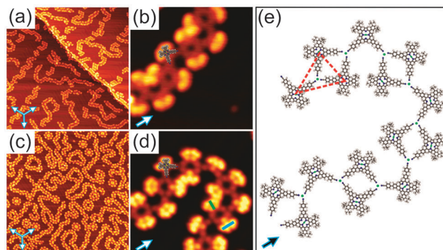
Fig. 2 (a and c) Overview STM images ( 150 \times 150 nm 2 ), showing the formation of 1D coordination polymers of 1 on Au(111) induced by annealing at 160^\circ\text{C} and deposition of Co, respectively. The set of three arrows indicates the principal directions of the underlying substrate. (b and d) Close-up STM images ( 15 \times 15 nm 2 ) for (a) and (c), respectively. Blue and green bars in (d) indicate A and B isomers, respectively. (e) The proposed model for the 1D coordination polymer of 1 on Au(111). The green dots in (e) represent Au atoms, while the red dashed triangle illustrates a basic unit of the 1D polymer. The STM images were taken at 77 K with U = -1.8 V, I = 20 pA.
