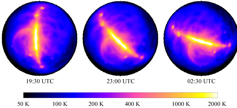
Figure 5.10: Images showing the apparent brightness temperature of the lunar surface at \nu = 60 MHz due to reflected Galactic and Extragalactic emission assuming specular reflection with a polarization independent albedo of 7%. The three panels correspond to 3 epochs at the beginning, middle, and end of the synthesis, the data for which is presented in this chapter.
