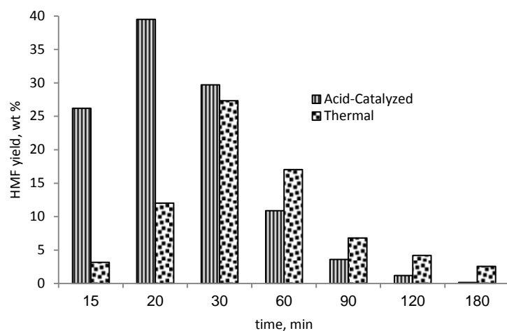
Fig. 10 HMF yield versus reaction time for the thermal and acid-catalysed conversion of inulin to HMF ( T=170^{\circ}\text{C} , C_{\text{in}}=0.17\text{ g/mL} , C_{\text{H}_2\text{SO}_4} = 0.006\text{ M} ).
