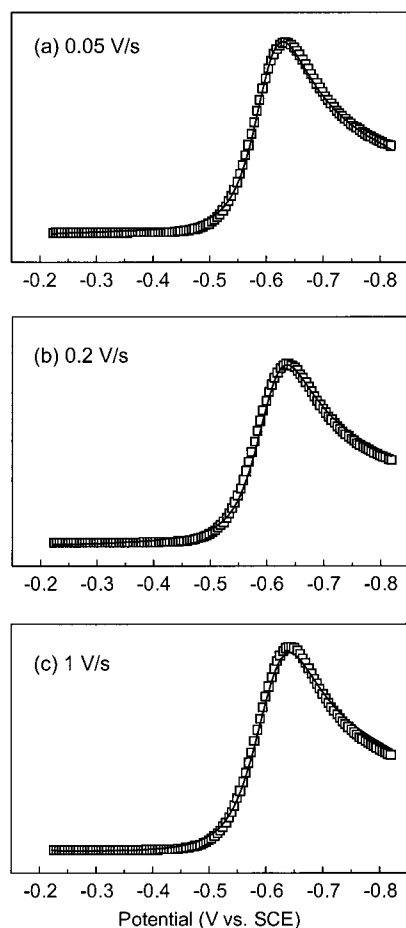
Figure 4. Scan rate variations of cyclic voltammograms by the experimental (—) and digital simulations ( \square ) of 0.15 mM QDI in \text{CHCl}_3/\text{CH}_3\text{CN} (4:1, v/v), (electrolyte: 0.1 M TBAPF 6 ): (a) = 0.05, (b) = 0.2, and (c) = 1 V/s at a 3.4 mm diameter Pt electrode. The experimental data were corrected for Ohmic drop. Simulation parameters: reduction reaction E_{1r} = -0.58 V vs SCE, E_{2r} = -0.62 V vs SCE, \alpha = 0.5 , k_s = 0.5 cm/s.
