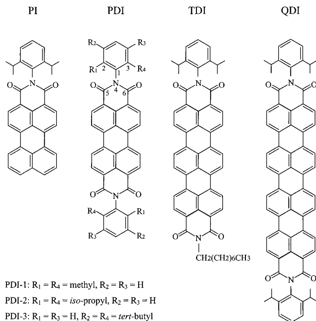
Figure 1. Chemical structures used in this investigation: PI, (2,6-diisopropylphenyl)-3,4-perylenedicarboxylic imide; PDI-1, N,N' -bis(2,6-dimethylphenyl)-3,4,9,10-perylenetetracarboxylic diimide; PDI-2, N,N' -bis(2,6-diisopropylphenyl)-3,4,9,10-perylenetetracarboxylic diimide; PDI-3, N,N' -bis(2,5-di- tert -butylphenyl)-3,4,9,10-perylenetetracarboxylic diimide; TDI, N -(2,6-diisopropylphenyl)- N' -octylterrylenetetracarboxylic diimide; QDI, N,N' -bis(2,6-diisopropylphenyl)-3,4,9,10-quaterrylenetetracarboxylic diimide.
