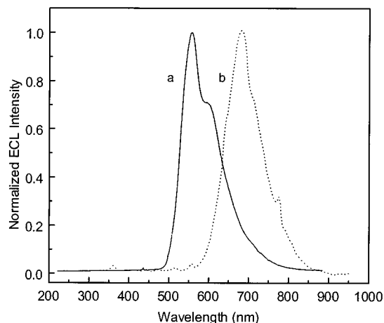
Figure 6. Normalized ECL spectra of (a) 8.0 \times 10^{-4} M PDI-2 in \text{CHCl}_3/\text{CH}_3\text{CN} (v/v, 3:2) and (b) 2.0 \times 10^{-4} M TDI in \text{CHCl}_3/\text{CH}_3\text{CN} (4:1, v/v). The potential was stepped (a) from -0.65 to +1.80 V and (b) from -0.80 to +1.40 V. The exposure time was 15 min (electrolyte: 0.1 M TBAPF 6 ).
