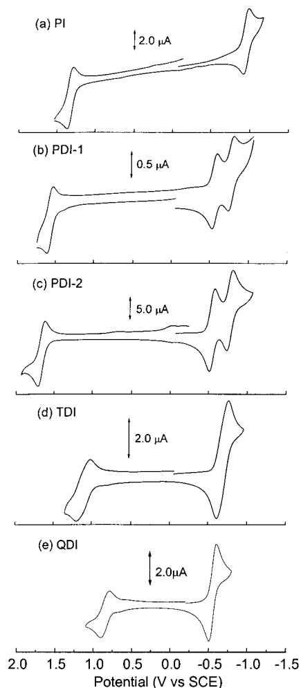
Figure 2. Cyclic voltammograms of (a) 0.8 mM PI in \text{CHCl}_3/\text{MeCN} (3:2, v/v), (b) 0.3 mM PDI-1 in \text{CH}_3\text{CN}/\text{MeCN} (2:1, v/v), (c) 0.8 mM PDI-2 in \text{CHCl}_3/\text{MeCN} (3:2, v/v), (d) 0.21 mM TDI in \text{CHCl}_3/\text{MeCN} (4:1, v/v), and (e) 0.1 mM QDI in \text{CHCl}_3/\text{MeCN} (4:1, v/v). Scan rate: (a, b) = 0.2 V/s; (c–e) = 0.5 V/s (electrolyte: 0.1 M TBAPF 6 ).
