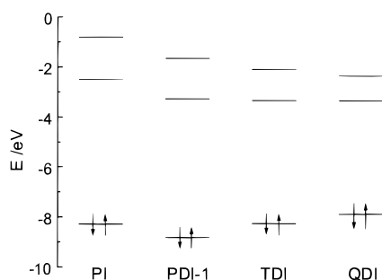
Figure 7. Molecular orbitals calculated with PM3.
