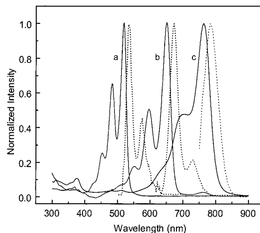
Figure 5. Normalized absorption (—) and fluorescence spectra (···) of (a) 1.0 \times 10^{-5} M PDI-1, (b) 1.0 \times 10^{-5} M TDI, and (c) 1.0 \times 10^{-5} M QDI in \text{CH}_3\text{Cl}/\text{CH}_3\text{CN} (3:2, v/v).
