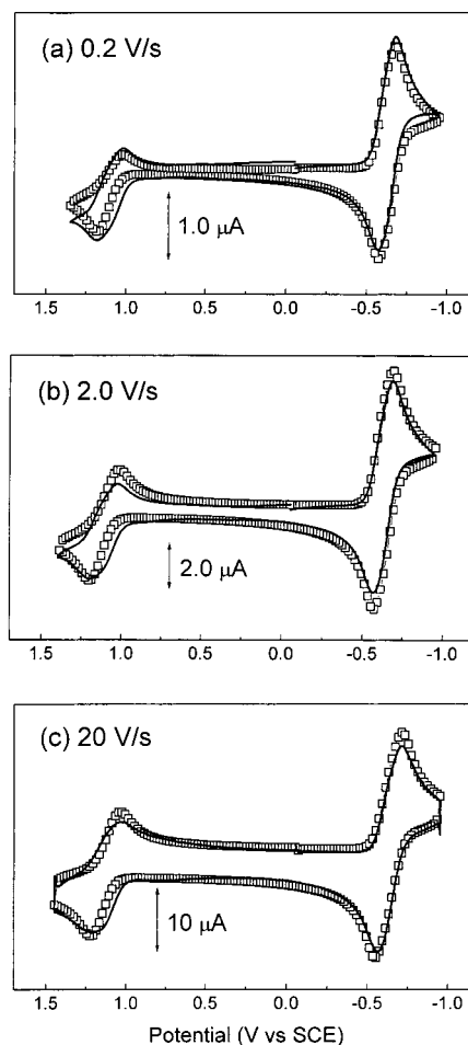
Figure 3. Scan rate variations of cyclic voltammograms by the experimental (—) and digital simulations (□) of 0.21 mM TDI in \text{CHCl}_3/\text{CH}_3\text{CN} (4:1, v/v), (electrolyte: 0.1 M TBAPF 6 ): (a) = 0.2, (b) = 2.0, and (c) = 20 V/s at a 1.4 mm diameter Pt electrode. The experimental data were corrected for Ohmic drop. Simulation parameters: reduction reaction E_{1r} = -0.63 V vs SCE, E_{2r} = -0.70 V vs SCE, \alpha = 0.5 , k_s = 1.0 cm/s; oxidation reaction E_{1o} = +1.21 V vs SCE, \alpha = 0.5 , k_s = 0.0035\text{--}0.05 cm/s, k_f = 0.1 s -1 .
