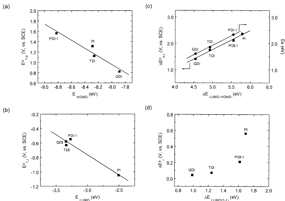
Figure 8. Correlation of experimental data with molecular orbital calculation results: (a) oxidation potential versus HOMO energy, (b) reduction potential versus LUMO energy, (c) potential difference between the first oxidation and first reduction waves versus energy difference between HOMO and LUMO, and (d) potential difference between the first and second reduction waves versus energy difference between the first and second LUMO.
