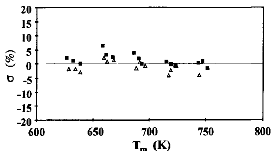
Fig. 7. \sigma as a function of T_m (model E). \varepsilon/\tau best-fit value = 0.124. Propane feed side: (■) tube; ( \Delta ) shell.
