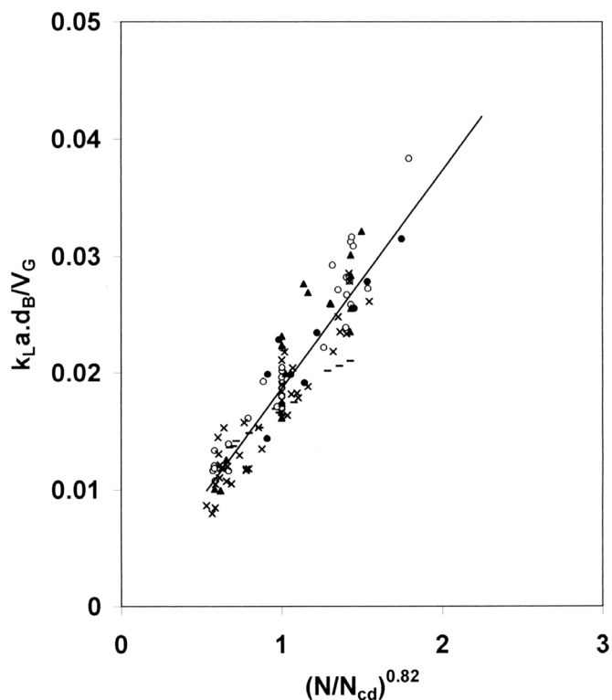
Figure 3. Correlating line plot for Equation (6). Legends: x; Data of Smith et al. (1977); •; Data of Chandrasekharan and Calderbank (1981); ▲; Data of Hickman (1988); o; Data of Smith (1991); -; Data of Whitton and Nienow (1993).
