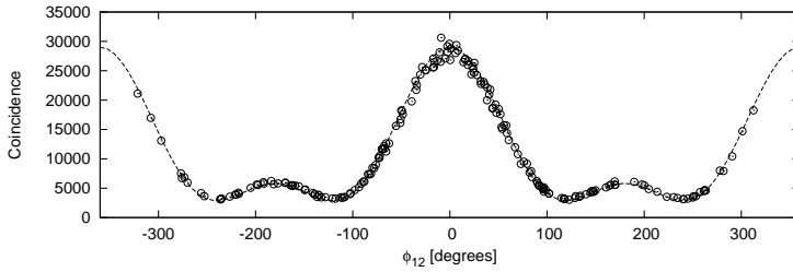
Figure 2.7: Case 3: Three particle correlation experiment (see Fig. 2.1 (bottom)). Simulation results of the three-particle coincidence counts as a function of \phi_{12} where \phi_{12} = \phi_1 - \phi_2 , and \phi_n = \phi_{A_n} - \phi_{B_n} ( n = 1, 2, 3 ). We only show data for the case \phi_{A_2} = \phi_{B_2} = 0 , \phi_{A_1} = \phi_{B_3} , \phi_{B_1} = \phi_{A_3} where \phi_{A_1} and \phi_{B_1} are chosen randomly. The time-of-flights of the messengers entering channel A and the time-of-flights of the messengers entering channel B are taken to be random (see text). Circles: Simulation data; Dashed line: Wave theoretical solution Eq. (2.9).
