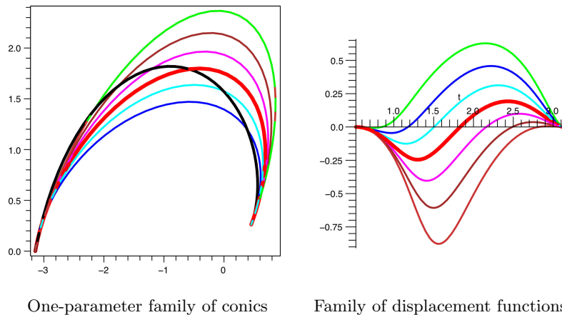
Figure 6.2: One-parameter family of bitangent conics and their corresponding displacement functions.
