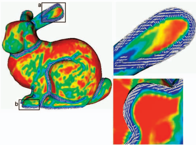
Fig. 7. In the vicinity of edges indicated by the combined classifier C_\epsilon^{0,1} , the feature directions based on the first moment M_\epsilon^1 are drawn. On the right-hand side, we zoom into the areas a and b, respectively.
