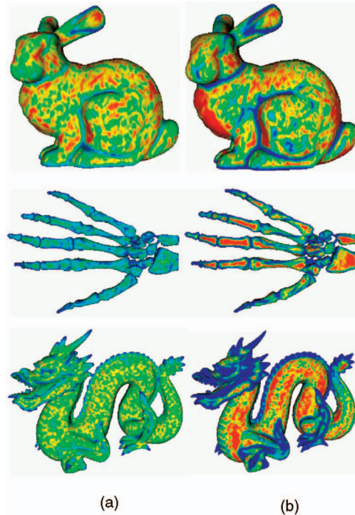
Fig. 6. Classifier applied to different surfaces. Left column: C_\epsilon^0 and right column: C_\epsilon^{0,1} .
