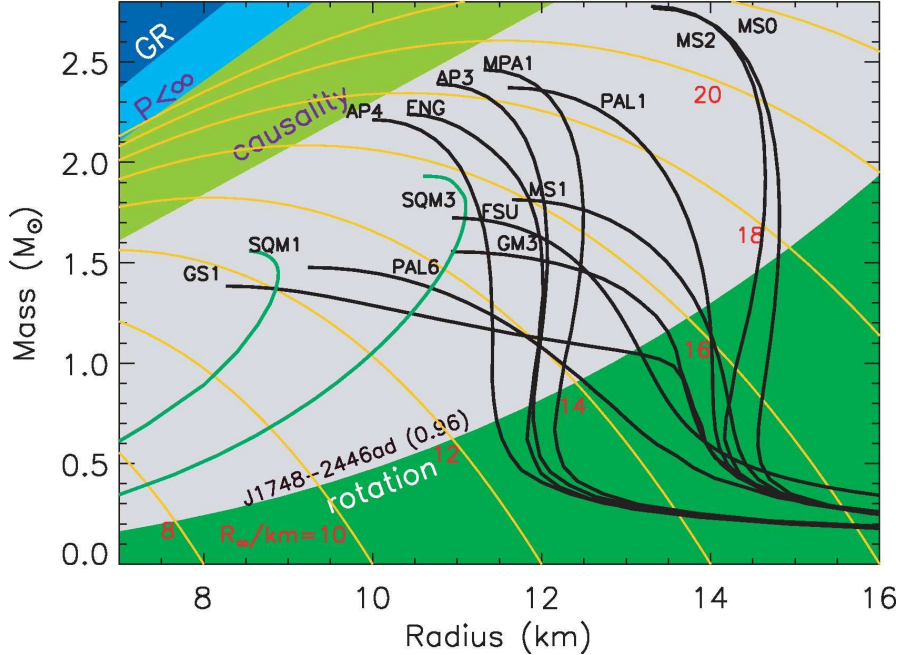
Figure 2: The mass-radius relationship for neutron stars reflects the equation of state for cold supdense matter. Mass-radius trajectories for typical EOSs are shown as black curves. Green curves (SQM1, SQM3) are self-bound quark stars. Orange lines are contours of radiation radius, R_\infty = R/\sqrt{1 - 2GM/Rc^2} . The dark blue region is excluded by the GR constraint R > 2GM/c^2 , the light blue region is excluded by the finite pressure constraint R > (9/4)GM/c^2 , and the light green region is excluded by causality, R > 2.9GM/c^2 . The green region in the right-hand corner shows the region R > R_{\max} excluded by the 716 Hz pulsar J1748-2446ad (Hessels et al. 2006). From Lattimer and Prakash (2007).
