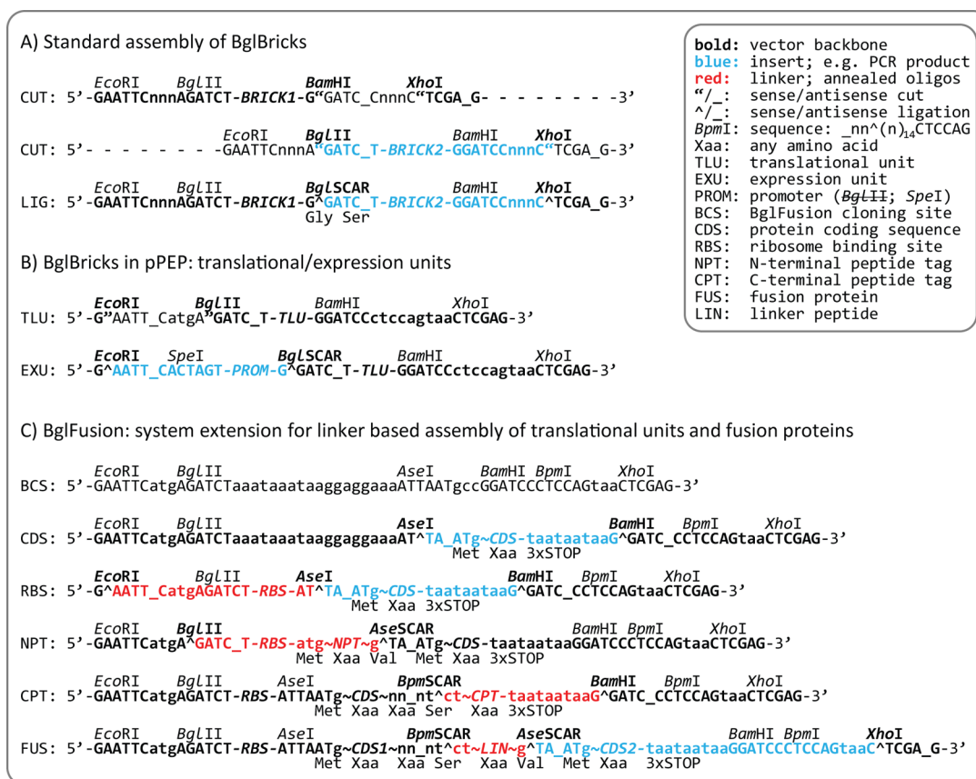
Figure 2. Functional unit assembly in pPEP1. BglBrick assembly was chosen as standard with its four restriction sites EcoRI , BglII , BamHI , and XhoI . Furthermore, the system was extended by the restriction sites AseI and BpmI to allow for an easy oligonucleotide-linker based exchange of RBSs, addition of peptide tags, or assembly of fusion proteins—the BglFusion format. Capital letters symbolize restriction recognition sites and bold restriction enzymes indicate positions where the backbone and inserts need to be cut and religated. Templates for the construction of oligonucleotide linkers are given in Table 1. Note that these are examples that suggest one way of how to assemble individual functional units and that alternatives are possible, offering maximal flexibility.
