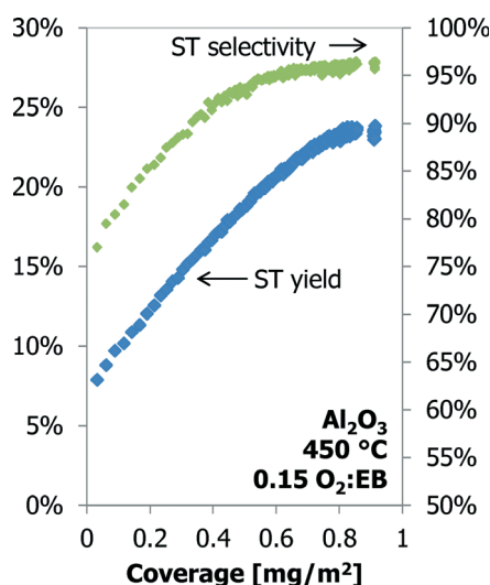
Fig. 9 The styrene yield and selectivity as a function of coke coverage for \text{Al}_2\text{O}_3 up to 70 h time-on-stream.
