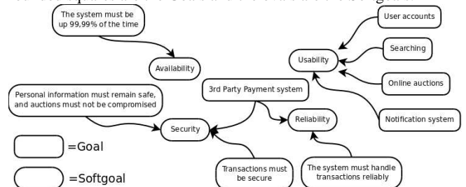
Fig. 7. Goal model.
