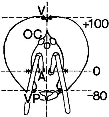
Fig. 1. Scheme of the basic orientation of the drone's head for the goniometer measurements. The zero position is given by an alignment of the antennal joints (A) with the binocular DPP positions (asterisks). The ventral point (VP) is at -80^\circ , the dorsal eye vertex (V) at +100^\circ elevation. OC: Ocelli.
