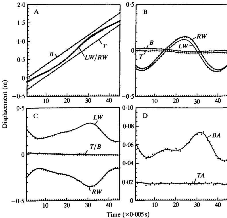
Fig. 2. (A–C) The position, digitized every 1/200 \text{ s} , of the beak ( B ), the tip of the tail ( T ) and the wing tips ( LW , RW ) of a male kestrel flying indoors at cruising speed over a mirror. Digitized points and fitted functions in the x - (A), the z - (B) and the y - (C) directions are drawn. (D) The projections on the horizontal plane of the total surface area of the bird ( BA ) and of the tail area ( TA ), with their fitted functions.
