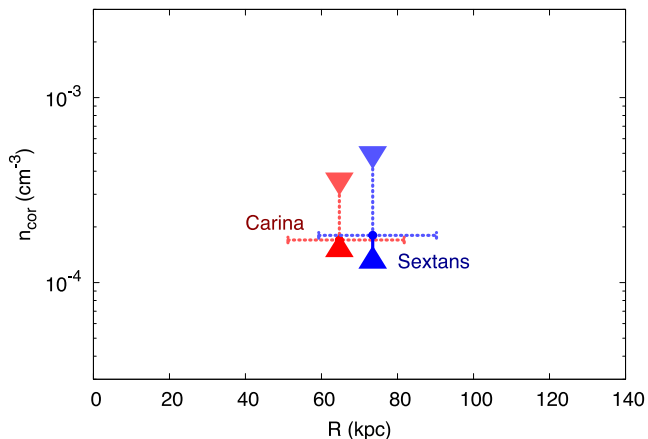
Figure 7. Ranges of gas densities of the MW's corona allowed by the Sextans (blue) and Carina (red) dwarfs. The derivation of the lower and upper bounds (triangles) is described in the text (Section 4.2).
