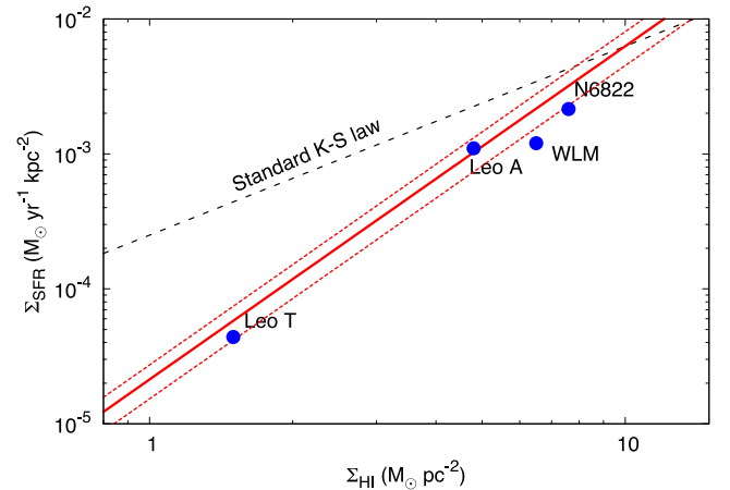
Figure 3. KS relation for dwarf galaxies as described by equation (10). The points show the location of four Local Group dIrrs (see Table 3).
