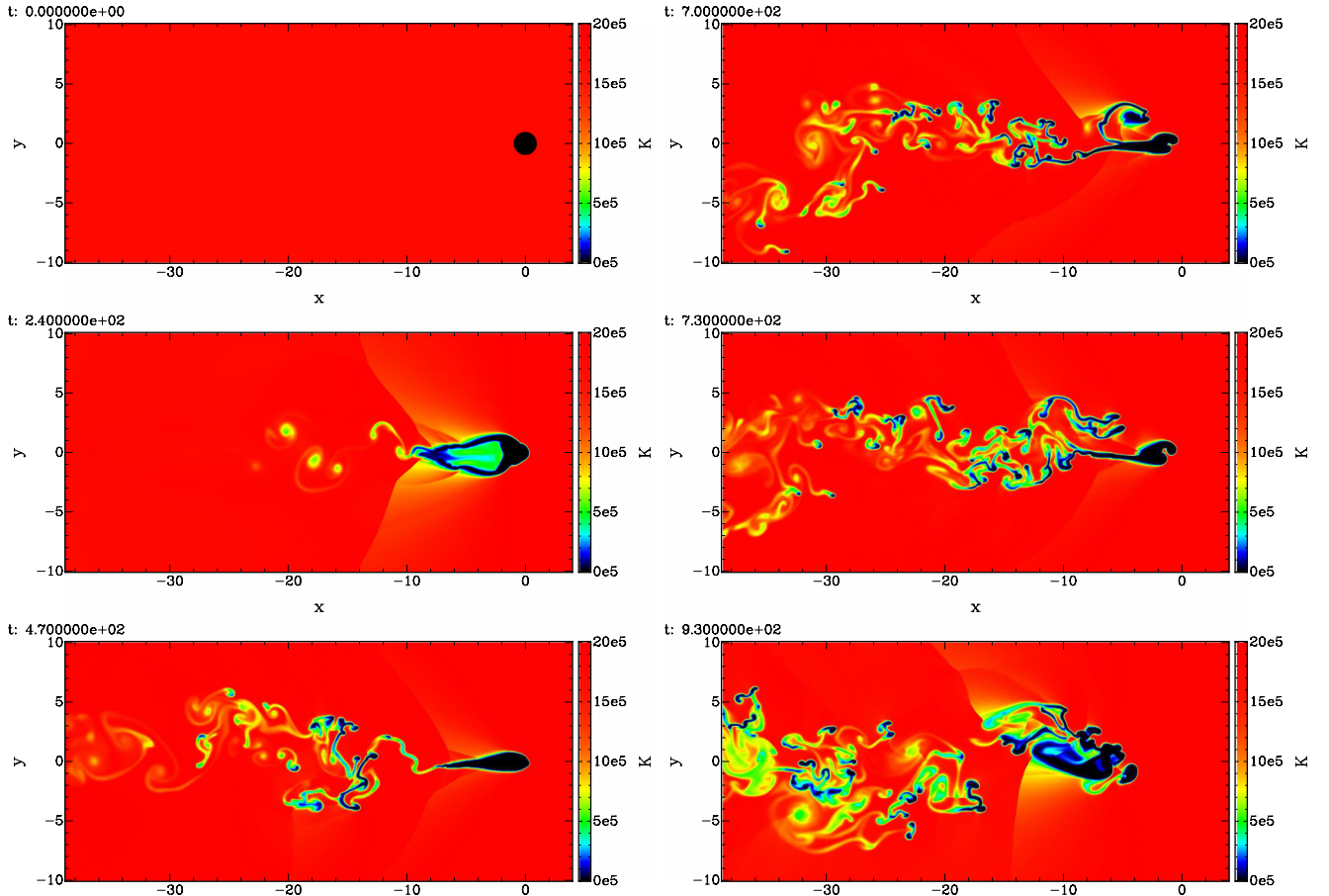
Figure 4. Time evolution of the temperature distribution for our fiducial setup for the Sextans dSph with n_{\text{cor}} = 1.8 \times 10^{-4} \text{ cm}^{-3} . In the left column (top to bottom), we show t = 0, 240 and 470 Myr, and in the right column we plot t = 700, 730 and 930 Myr. The bottom-left panel corresponds roughly to the time of pericentric passage. We only show a small section of the box. The axes are given in kpc.
