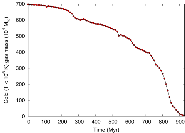
Figure 5. Mass of cold ( <10^5 K) gas gravitationally bound to the DM halo of Sextans as a function of time from the beginning of our fiducial simulation. The pericentre passage occurs at t = 465 Myr.
