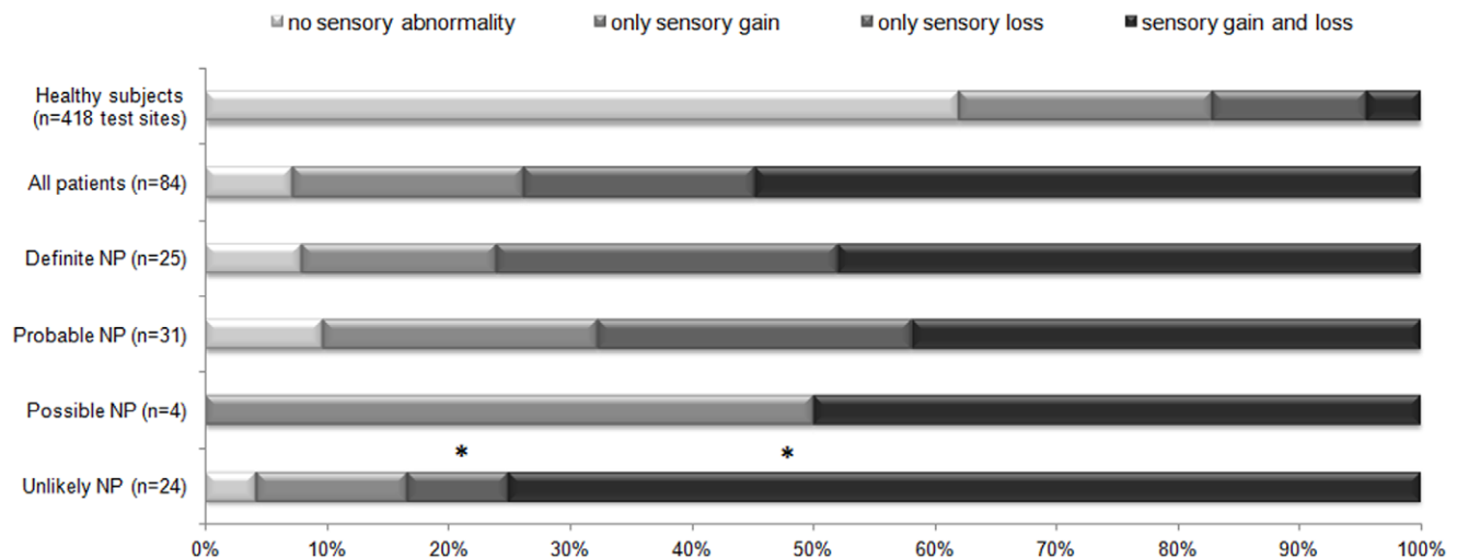
Figure 1. Sensory findings for patients according to neuropathic pain grades and healthy controls. Sensory findings (gain and/or loss of sensory function) in % for healthy controls ( n = 209 with 418 test sites), for patients ( n = 84 ) overall and ordered according to their likelihood to be neuropathic pain. “No sensory abnormalities”: none of the Quantitative Sensory Testing (QST) parameters were outside the 95% CI. “Only sensory gain”: at least one QST parameter indicating thermal or mechanical hyperesthesia or hyperalgesia without the presence of hypesthesia or hypoalgesia. “Only sensory loss”: at least one QST parameter indicating thermal or mechanical hypesthesia or hypoalgesia without the presence of hyperesthesia or hyperalgesia. “Sensory gain and loss”: at least one positive sign combined with one negative sign. Wilson estimates of proportions between the groups of definite and probable neuropathic pain and the group of unlikely neuropathic pain for only sensory loss and sensory gain and loss parameter ( *p < 0.05 ).
