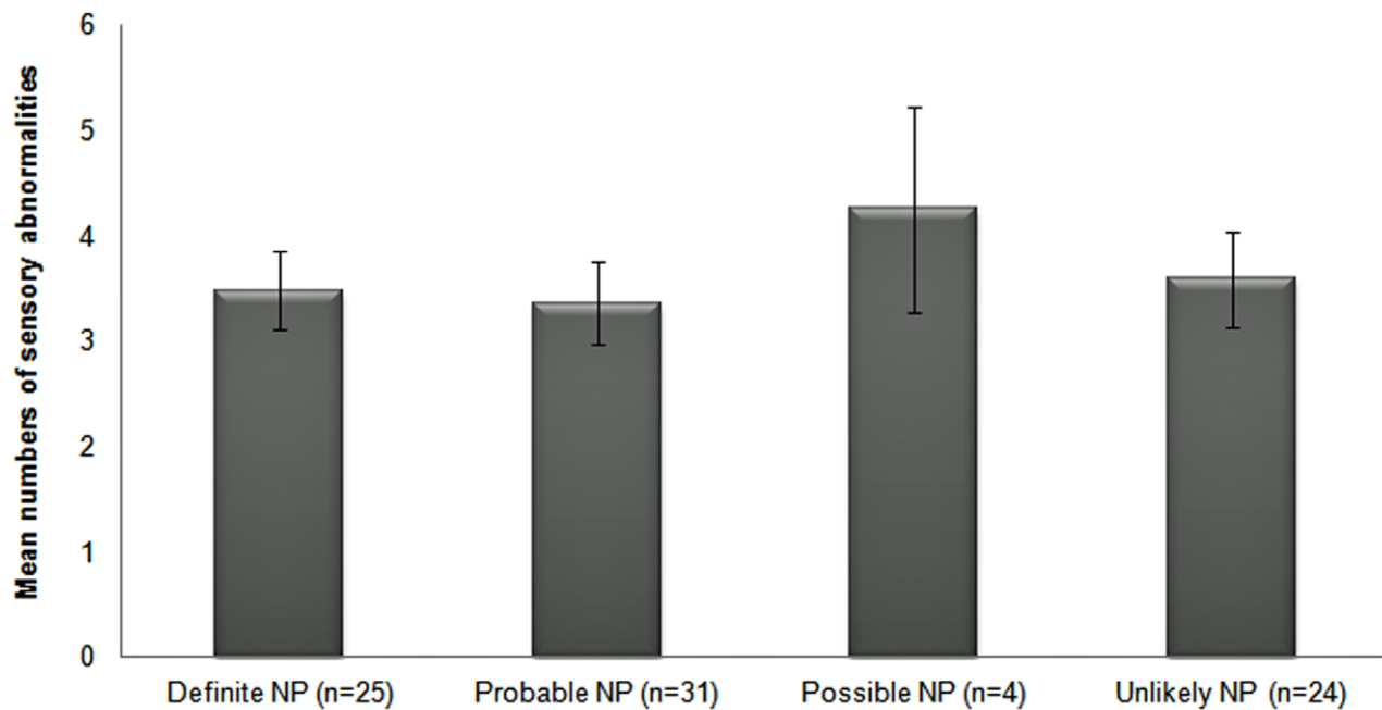
Figure 3. Numbers of sensory abnormalities for patients according to neuropathic pain grades. Numbers of sensory abnormalities (sensory gain and loss) for patients ( n = 84 ) graded as 'definite', 'probable', 'possible' and 'unlikely' neuropathic pain; Mean values \pm SEM. doi:10.1371/journal.pone.0043526.g003
