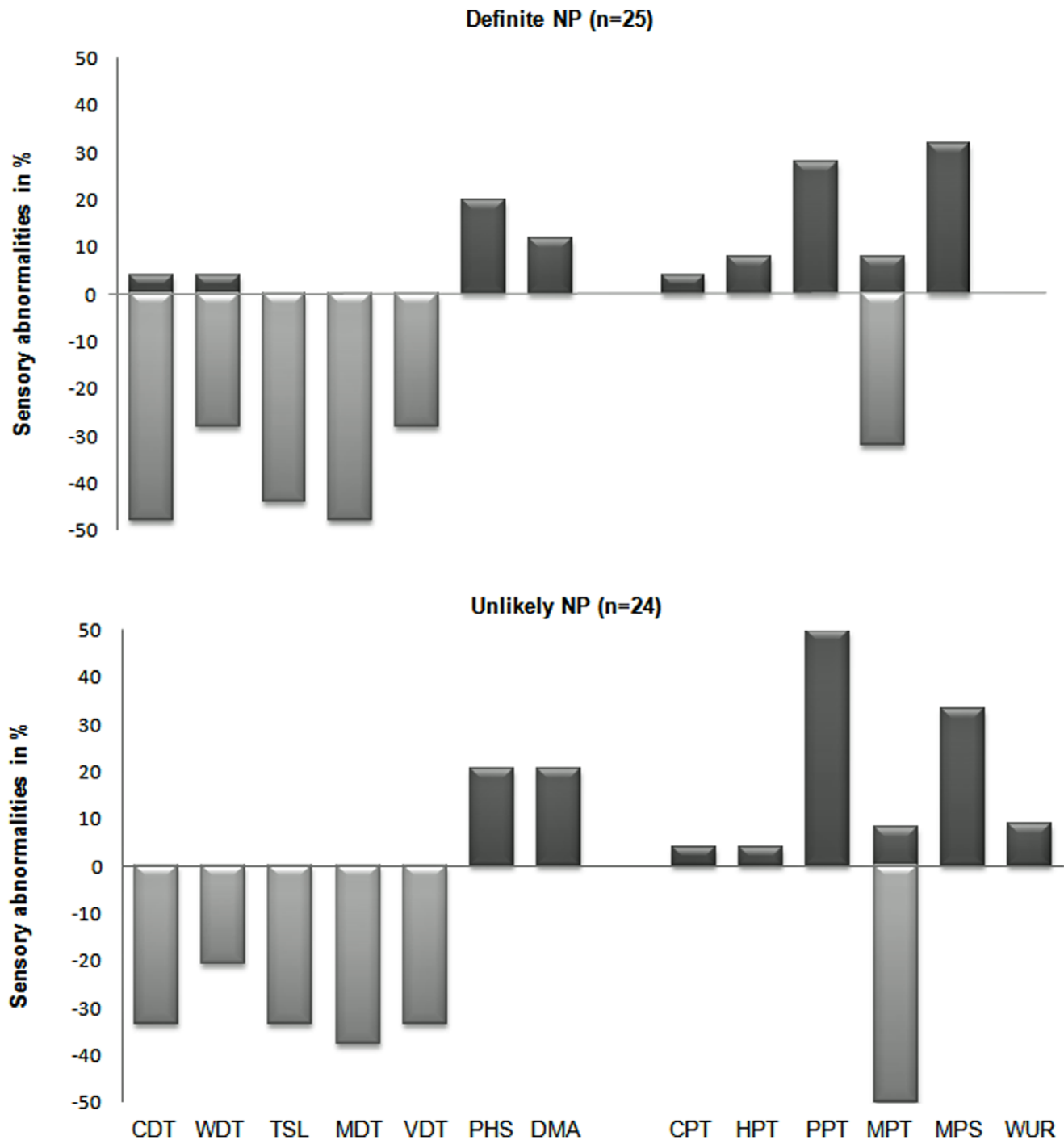
Figure 2. QST z-score abnormalities for patients graded as 'definite' and 'unlikely' neuropathic pain. Quantitative Sensory Testing (QST) z-score abnormalities in % for 'definite' neuropathic pain (top) and 'unlikely' neuropathic pain (bottom) grades. QST parameter are ordered as sensory parameters: Cold Detection Threshold (CDT), Warm Detection Threshold (WDT), Thermal Sensory Limen (TSL), Mechanical Detection Threshold (MDT), Vibration Disappearance Threshold (VDT), Paradoxical Heat Sensation (PHS), Dynamic Mechanical Allodynia (DMA) and nociceptive parameters: Cold Pain Threshold (CPT), Heat Pain Threshold (HPT), Pressure Pain Threshold (PPT), Mechanical Pain Threshold (MPT), Mechanical Pain Sensitivity (MPS) and Wind Up Ratio (WUR). Z-scores with positive sensory signs (gain of sensory function) plotted upwards and negative sensory signs (loss of sensory function) plotted downwards. Absence of DMA is normal and therefore no negative sign possible. doi:10.1371/journal.pone.0043526.g002
