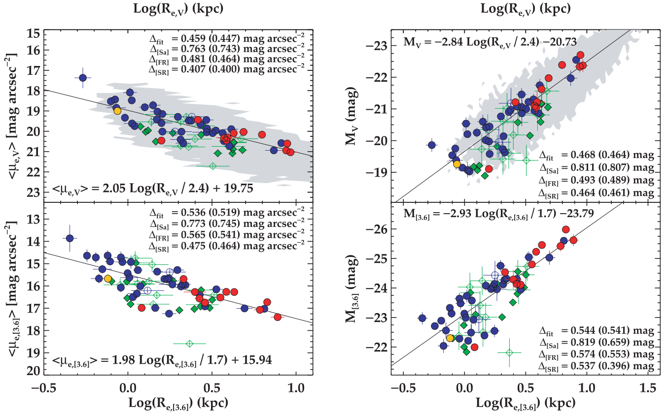
Figure 8. KR and SLR for the galaxies in the SAURON sample in the V and 3.6\text{-}\mu\text{m} bands. Symbols are as in Fig. 3. The thick solid line is the best-fitting relation (as indicated in the equation in each panel). \Delta_{\text{fit}} indicates the observed and intrinsic scatters (the latter in parentheses) for the galaxies used to obtain the fit, while \Delta_{[\dots]} represent the measured values for the different families around the best-fitting relations. The grey area marks the extent of the B03 sample.
