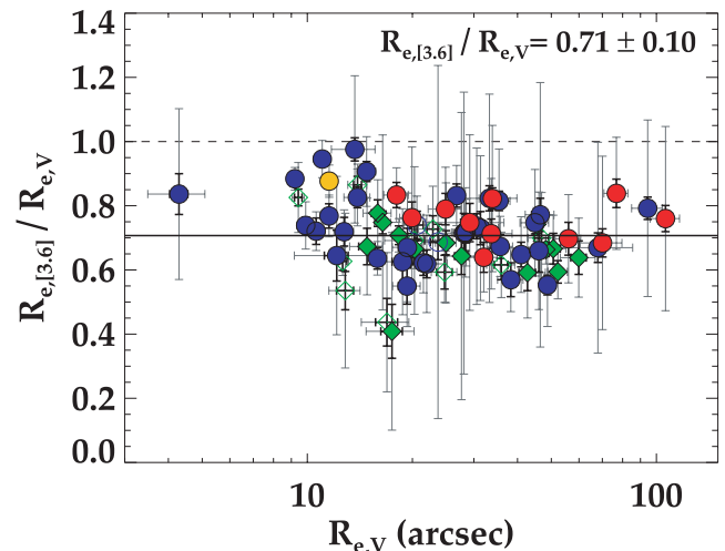
Figure 3. Ratio between R_{e,V} and R_{e,[3.6]} for our sample of galaxies. The solid thick line shows the average ratio ( R_{e,[3.6]}/R_{e,V} ). The dashed line marks the one-to-one relation. The circles denote E/S0 galaxies and the diamonds denote Sa galaxies. The filled symbols indicate galaxies with good distance estimates and open symbols indicate those with only recession velocity determinations. In blue, we highlight FRs, in red, SRs, and in green, the Sa galaxies. The special case of NGC 4550, with two similarly-massive counter-rotating disc-like components, is marked in yellow. The black/grey error bars denote the minimum/maximum uncertainties in our analysis (see Section 4.1).
