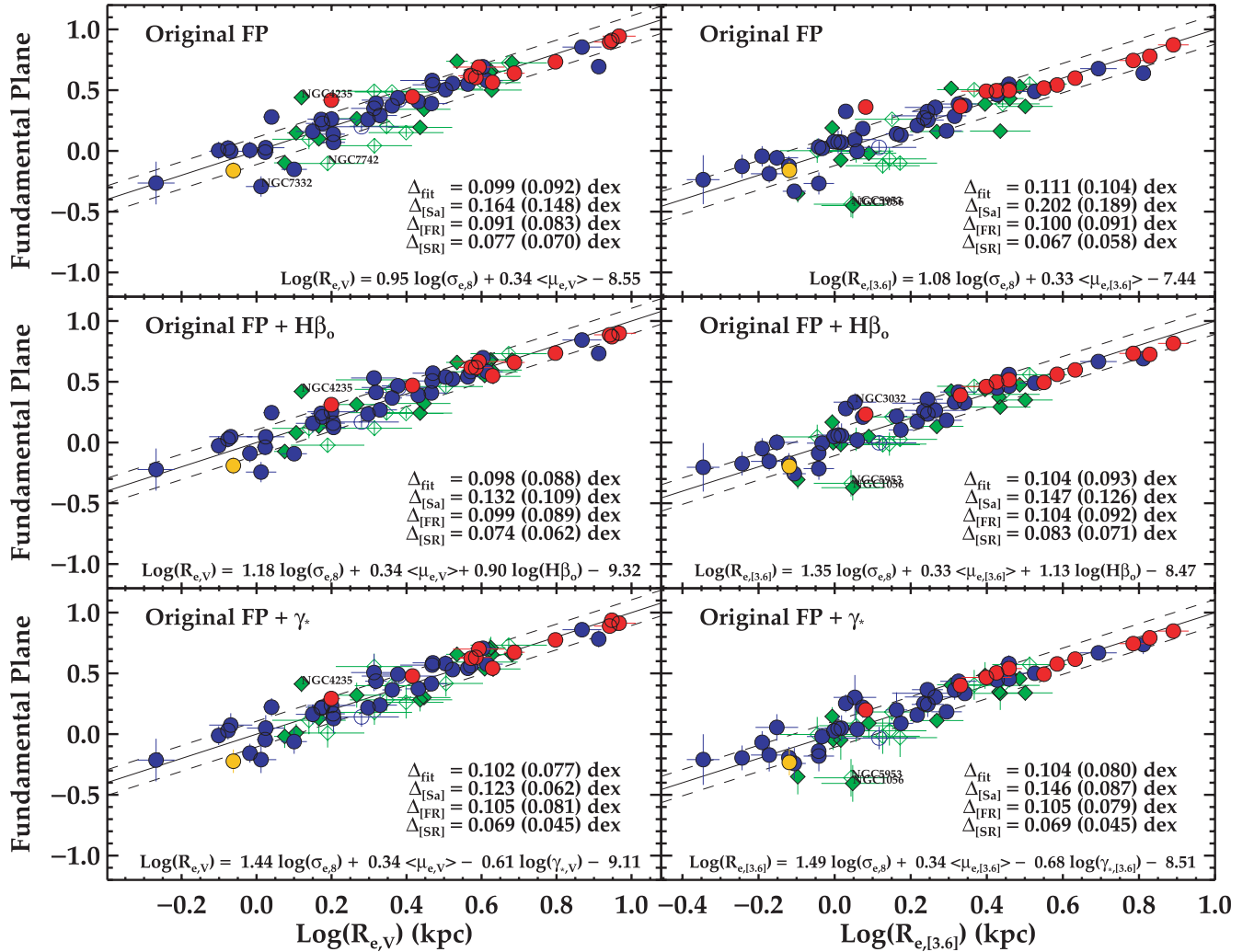
Figure 15. Edge-on views of the FP relations for the galaxies in the SAURON sample in the V and 3.6\text{-}\mu\text{m} bands. Here \sigma_e/8 ( \sigma_{e,8} ) is used instead of \sigma_e . Symbols are as in Fig. 3. Top row: original FP relation. Middle row: original FP relation with an \text{H}\beta_0 term. Bottom row: original FP relation with a \gamma_* term. The dashed lines mark the 1\sigma uncertainty [measured in \log(R_e) ] considering all objects. The solid line is the best-fitting relation (as indicated in the equation in each panel). \Delta_{\text{fit}} indicates the observed and intrinsic scatters (the latter in parentheses) measured along the \log(R_e) axis for the galaxies used to obtain the fit, while \Delta_{[\dots]} represent the measured values for the different families around the best-fitting relations.
