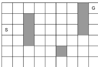
Figure 3: The Dyna Maze task, in which the agent must travel from S to G . The reward is +1 when the goal state is reached and 0 otherwise.
