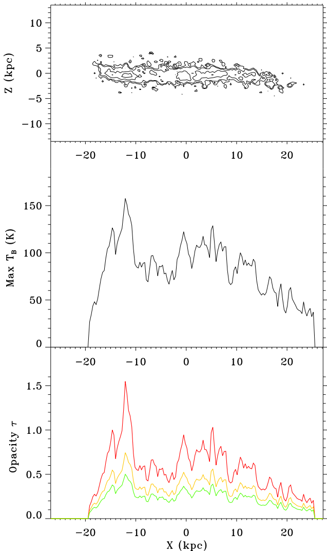
Fig. 4c. ESO138-G014. Top : Peak brightness temperature map. Countours are plotted in (41, 51, 83, 124) \times \sigma , where the rms noise is 10.4 K. The FWHM synthesised beam has dimensions 10.7'' \times 10.7'' . Middle: Major axis peak brightness temperature profile. Bottom: Inferred HI opacity calculated assuming constant HI spin temperatures. The resulting maximum opacities along each line of sight column through the galaxy disk are plotted for T_{spin} = 200, 300 and 400 K (bottom to top).
