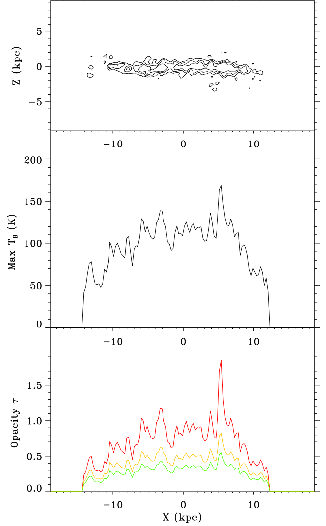
Fig. 5c. ESO146-G014. Top : Peak brightness temperature map. Contours are plotted in (60, 80, 100) \times \sigma , where the rms noise is 14.9 K. The FWHM synthesised beam has dimensions 7.6'' \times 7.6'' . Middle: Major axis peak brightness temperature profile. Bottom: Inferred HI opacity calculated assuming constant HI spin temperatures. The resulting maximum opacities along each line of sight column through the galaxy disk are plotted for T_{spin} = 200, 300 and 400 \text{ K} (bottom to top).
