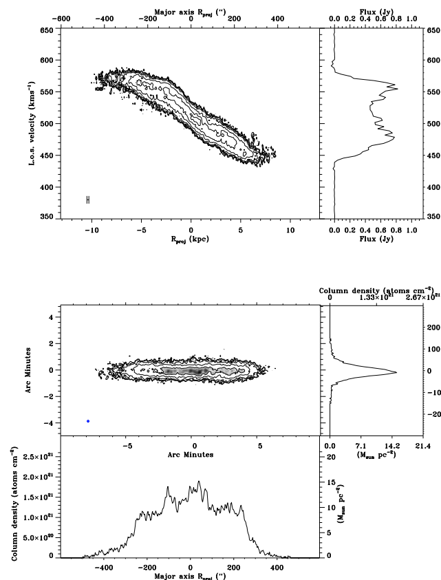
Fig. 3b. ESO115-G021. Top left: XV map. XV contours are (3, 5, 10, 20, 50, 100, 150) \times \sigma , where the rms noise \sigma = 1.55 \text{ mJy beam}^{-1} or 2.16 \times 10^{19} \text{ atoms cm}^{-2} . The half power beam extent over the major axis is shown in the lower left corner. Top right: Integrated spectrum. Middle left: HI column density map rotated with the galaxy major axis aligned with the X axis. Column density map contours are (3, 5, 10, 25, 50) \times \sigma , where the rms noise \sigma = 1.47 \text{ mJy beam}^{-1} or 2.04 \times 10^{19} \text{ atoms cm}^{-2} . The FWHM synthesised beam has dimensions 8.9'' \times 8.9'' , and is displayed as a cross-hatched symbol in the lower left. Middle right: Minor axis profile. Bottom left: Major axis profile.
