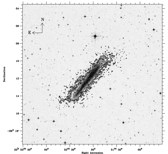
Fig. 1a. ESO074-G015 (IC5052). HI column density map overlaid on the DSS image. Contours are plotted in (3, 5, 10, 25, 50, 80) \times \sigma , where the rms noise \sigma = 2.05 mJy beam -1 or 2.79 \times 10^{19} atoms cm -2 . The FWHM synthesised beam has dimensions 9.0'' \times 9.0'' , and is displayed as a cross-hatched symbol in the lower left.
