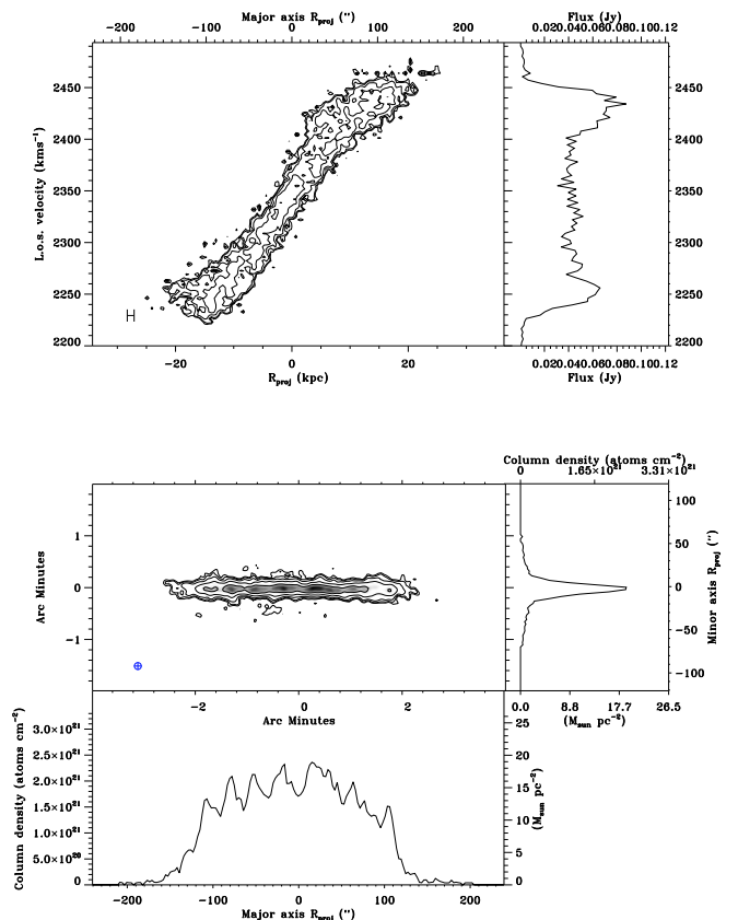
Fig. 2b. ESO109-G021 (IC5249). Top left: XV map. XV contours are (3, 5, 10, 20, 40) \times \sigma , where the rms noise \sigma = 1.76 \text{ mJy beam}^{-1} or 3.03 \times 10^{19} \text{ atoms cm}^{-2} . The half power beam extent over the major axis is shown in the lower left corner. Top right: Integrated spectrum. Middle left: HI column density map rotated with the galaxy major axis aligned with the X axis. Column density map contours are (3, 5, 10, 25, 50) \times \sigma , where the rms noise \sigma = 1.62 \text{ mJy beam}^{-1} or 2.79 \times 10^{19} \text{ atoms cm}^{-2} . The FWHM synthesised beam has dimensions 8.0'' \times 8.0'' , and is displayed as a cross-hatched symbol in the lower left. Middle right: Minor axis profile. Bottom left: Major axis profile.
