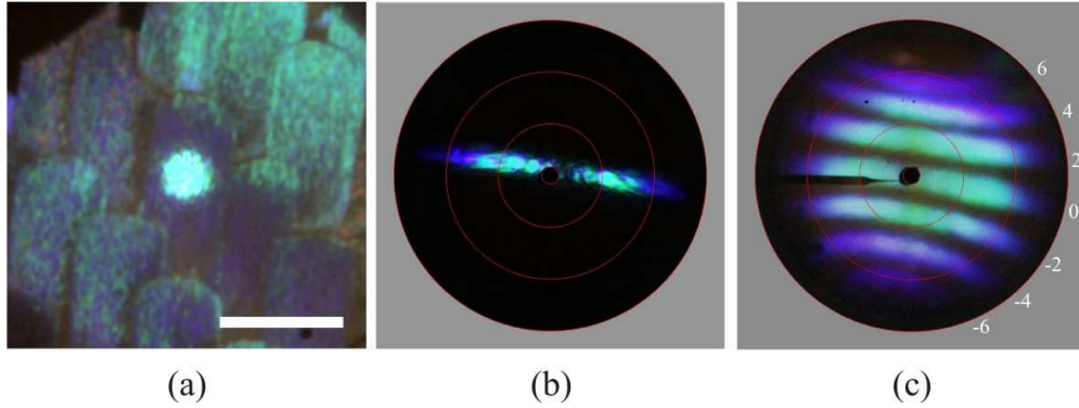
Fig. 4. Scattering by a dorsal wing scale of the butterfly Morpho aega . (a) A small wing fragment was positioned in the scatterometer and the primary beam was projected as a 40\ \mu\text{m} spot at a single scale (a much wider area was illuminated by a weaker beam delivered by the secondary source); bar 100\ \mu\text{m} . (b) The scattering pattern resulting from the primary beam. (c) Scattering patterns created by the secondary beam with diaphragm D_4 positioned at d = 0, \pm 2, \pm 4, and \pm 6 mm with respect to the axis (corresponding to an angle of incidence of \theta_i = 0^\circ, \pm 20.5^\circ, \pm 39.9^\circ and \pm 57.1^\circ , respectively). The long, pointed, black object at 9 o'clock is the glass micropipette holding the about circular wing fragment. The red circles in (b) and (c) indicate scattering angles of \theta_s = 5, 30, 60, and 90 degrees.
