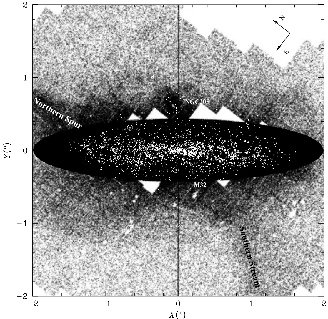
Figure 1. Composite illustration of the data on the star stream in M31, presented in a coordinate system in which X lies along the major axis of M31, increasing toward the SW, Y increases along the minor axis toward the NW, and Z increases along the line of sight. The greyscale shows the star-count data, as published in Ferguson et al. (2002), with the Southern Stream and Northern Spur annotated. The black ellipse indicates the extent and inclination of M31's disc, and the locations of NGC 205 and M32 are also marked. The points show the PNe detected in the PN.S survey, with the size of the symbols encoding their line-of-sight velocities relative to M31 (crosses receding, boxes approaching). The circled points are 'friendless' PNe that lie more than 4\sigma in velocity from their 30 nearest neighbours.
